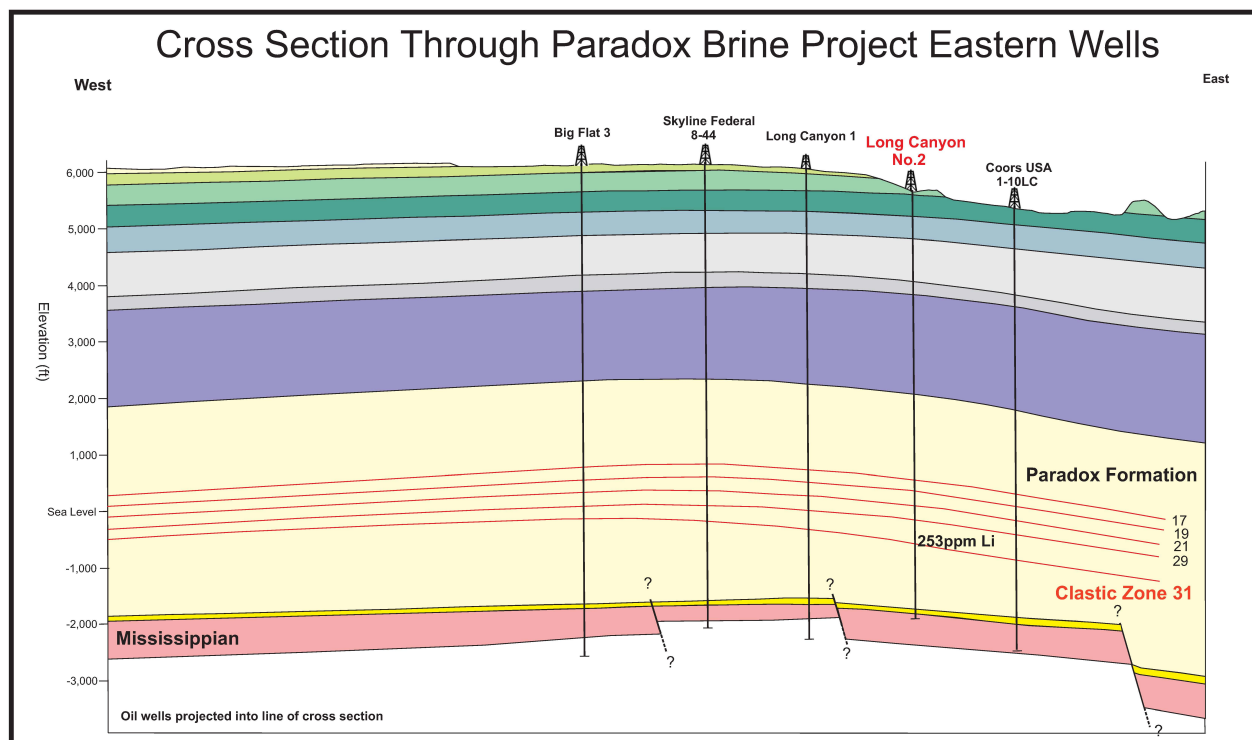
Figure 1: East-West Cross section showing the thickness of the Mississippian target units.
