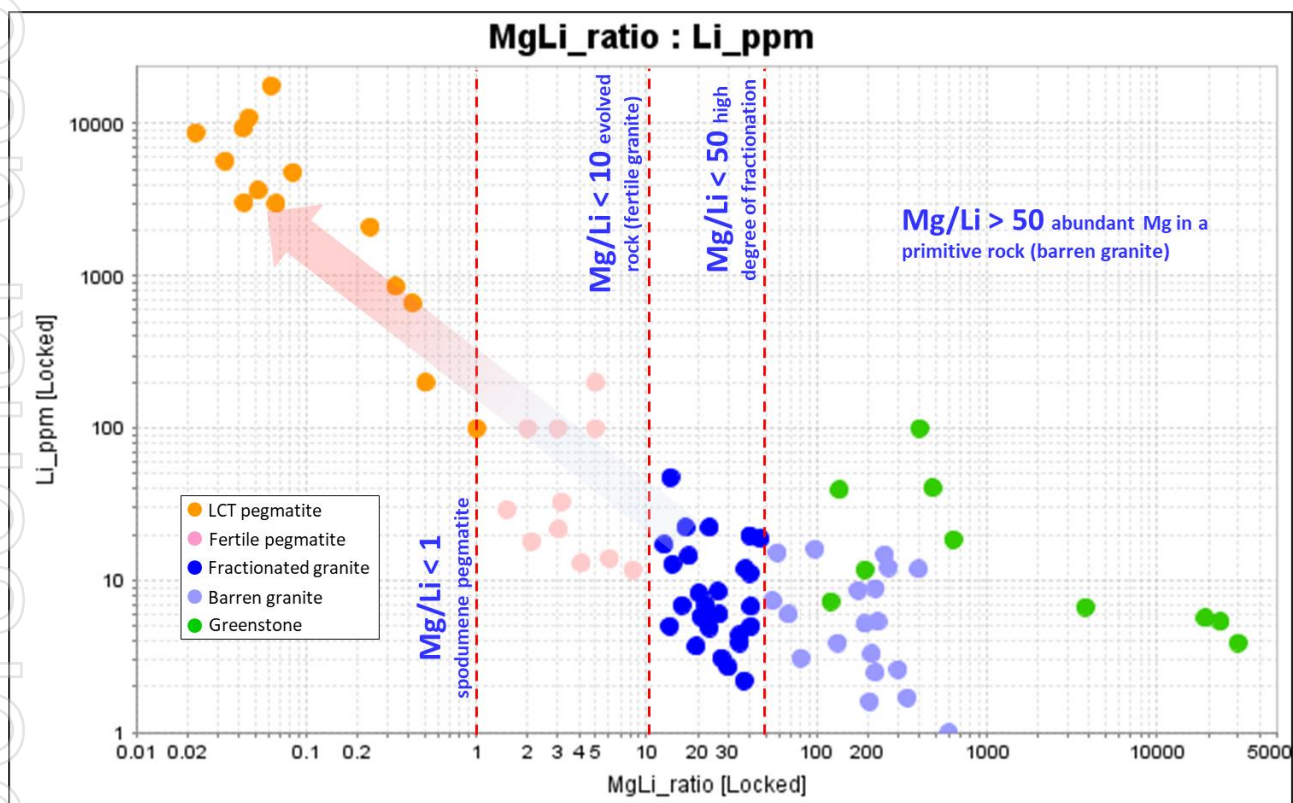
Figure 3: Li vs Mg/Li LCT rock classification graph for rock chips collected by Wildcat and Fairplay Gold across the Wildplay JV area showing a profound trend towards enriched spodumene LCT pegmatite. Sample locations and assays listed in Appendix 2 and shown on Figure 6 in Appendix 3.
