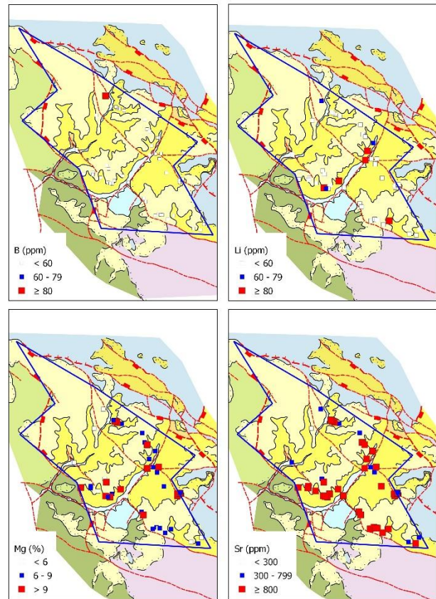
Figure 3 – Dobrinja project geology map with rock sampling positions and Li, B, Mg and Sr values
