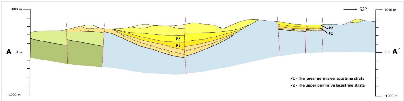
Figure 2 – Dobrinja cross section indication lateral extension of permissive lacustrine strata
