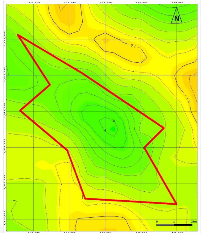
Figure 4 –Bouguer gravity image contoured at 1 mGal
