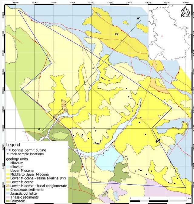
Figure 1 – Dobrinja project geology map
