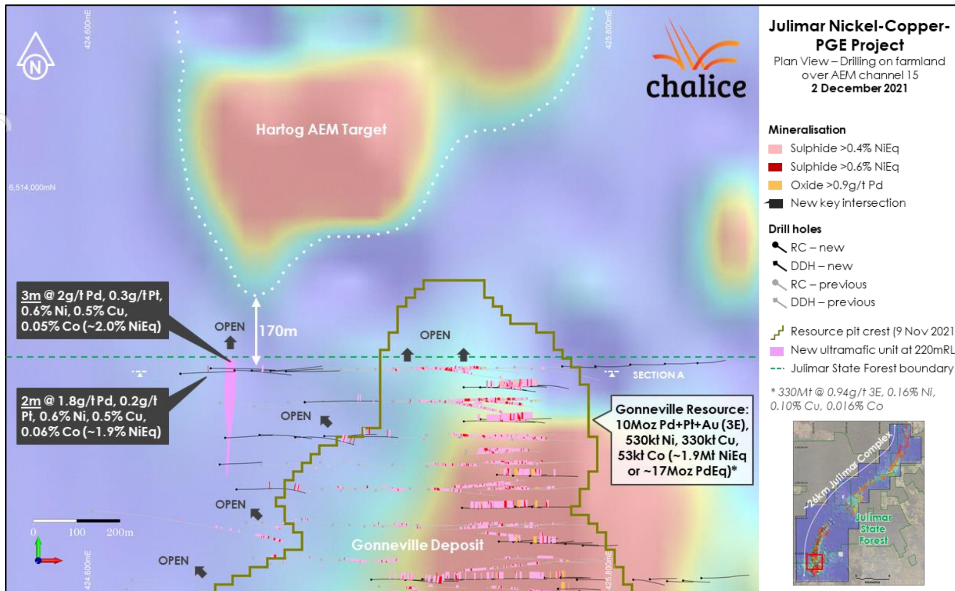
Figure 2. Gonneville north and Hartog south Plan View – drilling results and Resource pit crest over ch15 Airborne EM.
