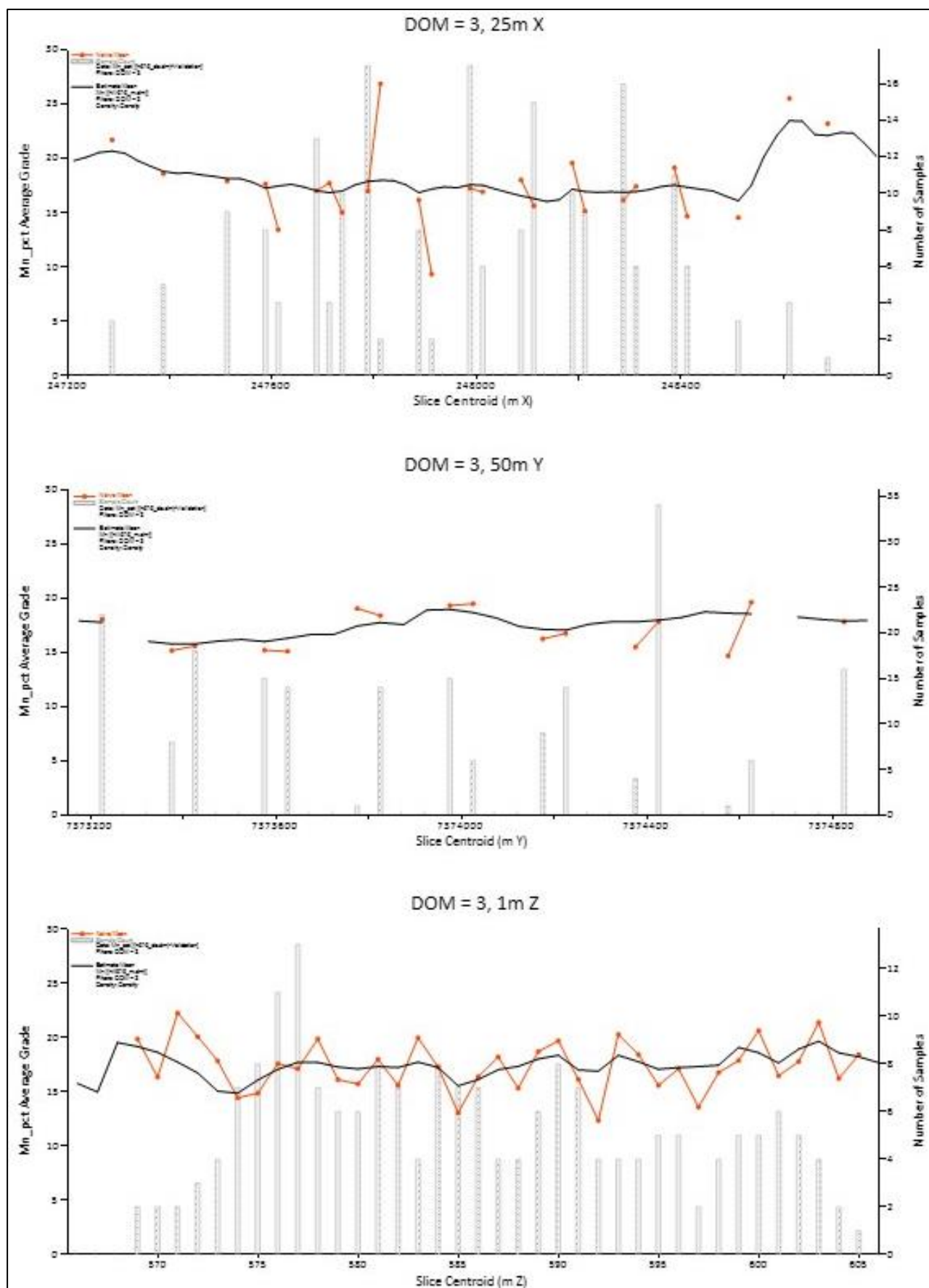
Figure 12: Comparison of the supergene manganese (Domain 3) Mn grades along northing, easting and elevation
