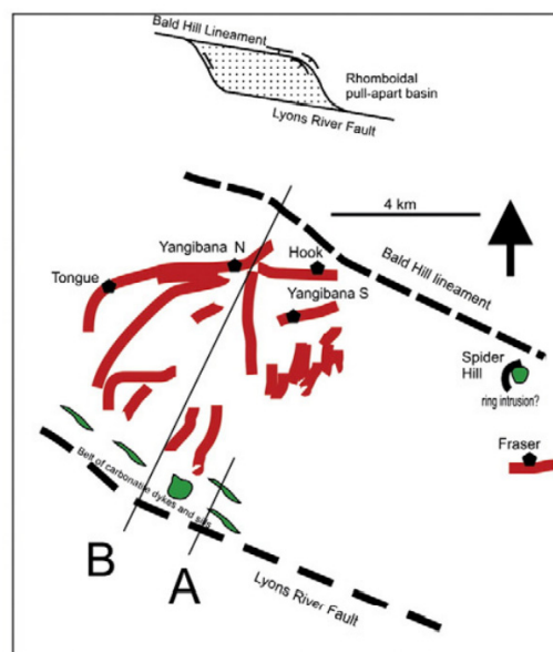
Figure 4. Two-stage model for the emplacement of ferrocarnatite sills and dykes at ~1075 Ma along Lyons River Fault (A), followed by strike-slip movements, formation of a pull-apart structure and emplacement of carbonatite-ironstone veins swarm at ~1050 Ma (B); bottom panel shows a schematic spatial distribution of the 1075 Ma ferrocarnatites dykes and sill and the adjacent 1050 Ma Fe oxide veins swarm emplaced in a pull-apart structure formed during re-activation of the Lyons River Fault; lines A and B in this panel schematically represent the two cross-sections above.
