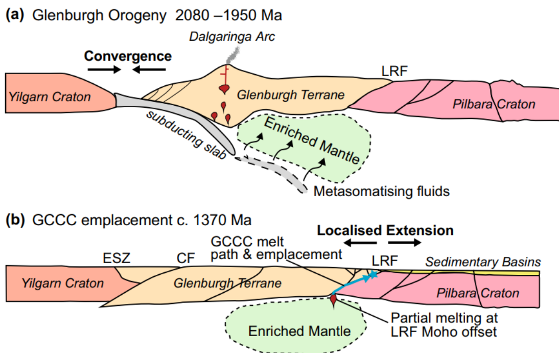
Figure 3. a) Mantle metasomatism under the Glenburgh Terrane resulting from plate subduction during the Glenburgh Orogeny (2080–1950 Ma). b) Localised extension caused minor decompression melting at the Lyons River Fault Moho offset, creating the alkaline melts that travel along the fault and are emplaced as the GCCC. CF Cardilya Fault, ESZ Errabiddy Shear Zone, LRF Lyons River Fault. Modified from Johnson et al. (2011, 2013).
