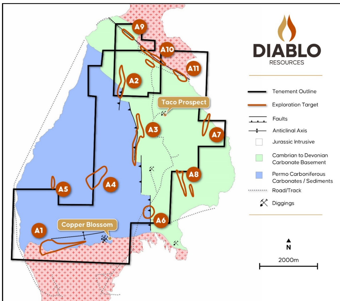
Figure 3 - Western Desert Project- Geology and Prospect Location Map
