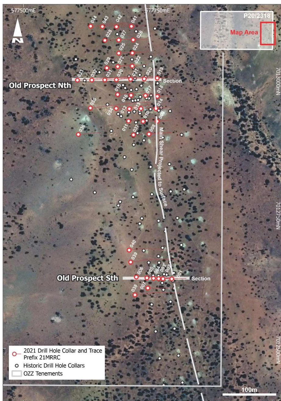
Figure 6: Drill Hole Plan
