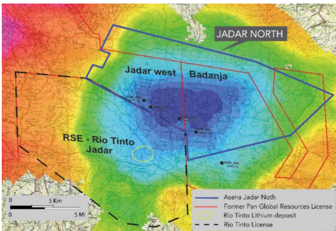
Figure 4: 2012 gravity field survey completed for the former Jadar West and Bandanja projects which now fall largely in Jadar North's licence application area
