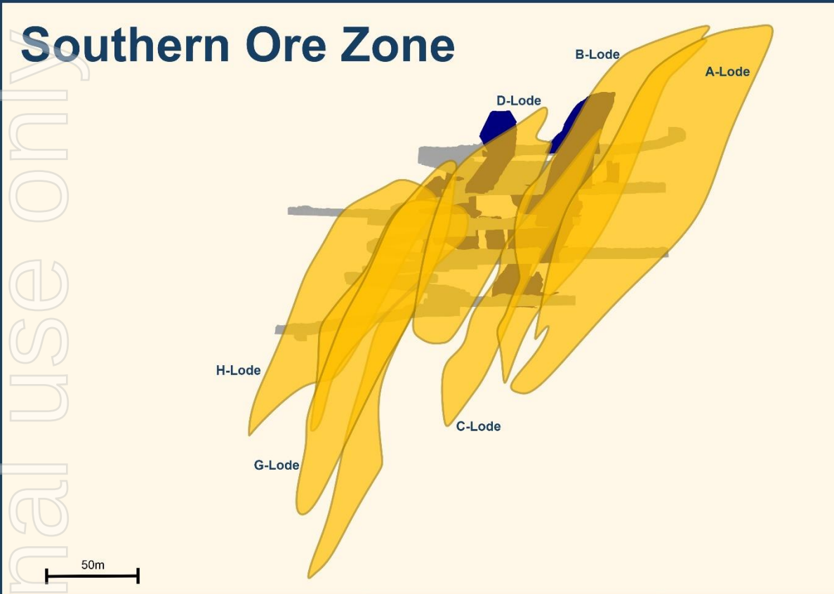
Cross Section of SOZ showing mineralisation domains and previous stopeing
