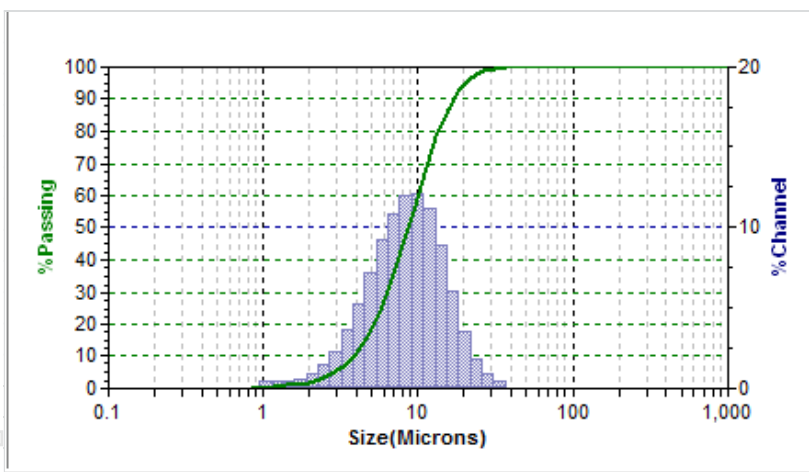
Particle Size Distribution of Spheroidisation Process Rejects with Volt’s Bunyu Natural Flake Graphite
