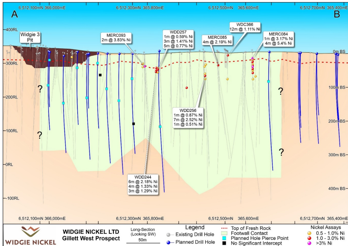
Figure 5: Long section of Gillett West looking southwest
