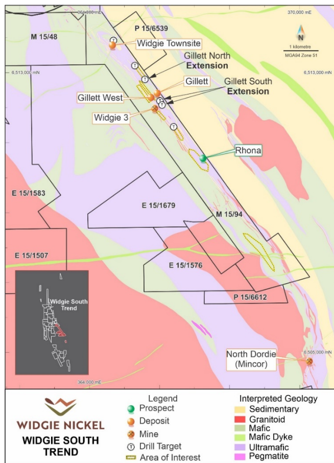
Figure 1: Widgie South deposits, located on the northeast margin of the Widgiemooltha Dome
