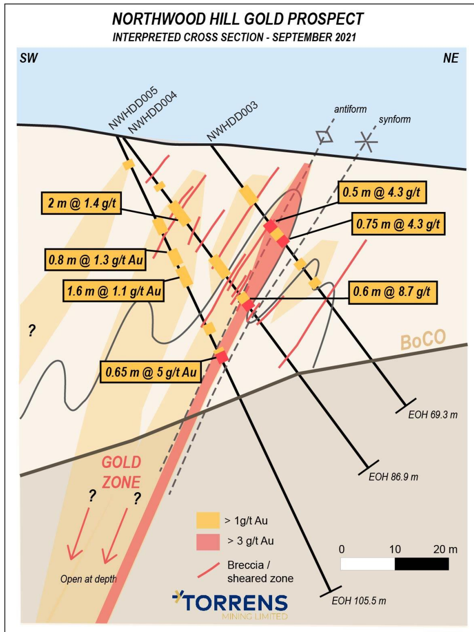
Figure 3 – Cross section showing the interpreted tightly folded anticlines and the location of gold mineralisation (BoCO = Base of Complete Oxidation)
