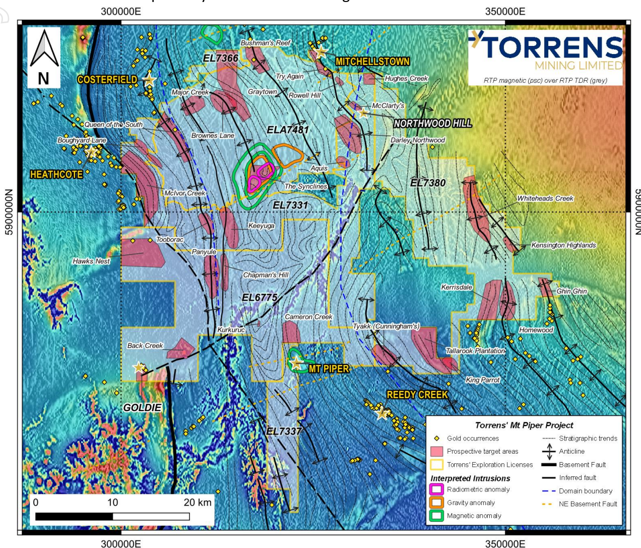
Figure 5 – Mt Piper Regional Targets and Structural Trends Overlying Project Magnetics
