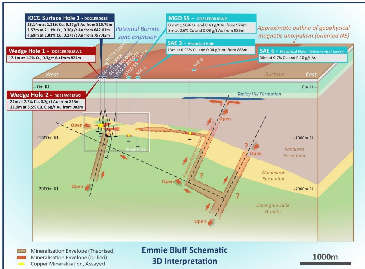
Figure 6 – 3D Schematic Interpretation of Emmie Bluff IOCG and Copper-Cobalt Mineralisation Setting
