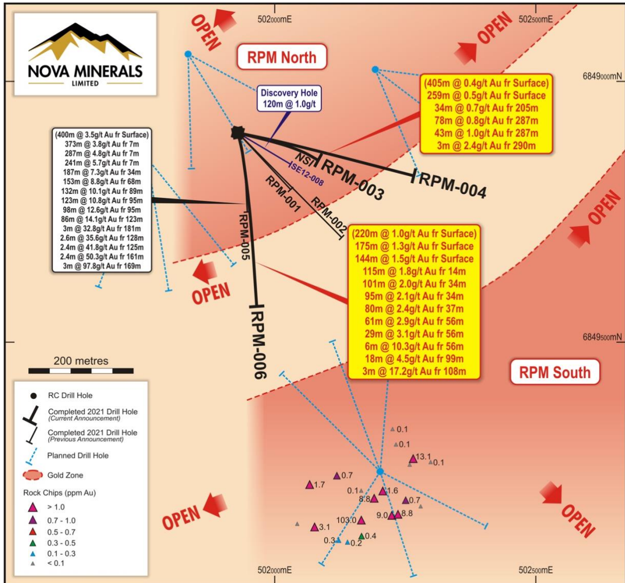
Figure 2. Plan View
