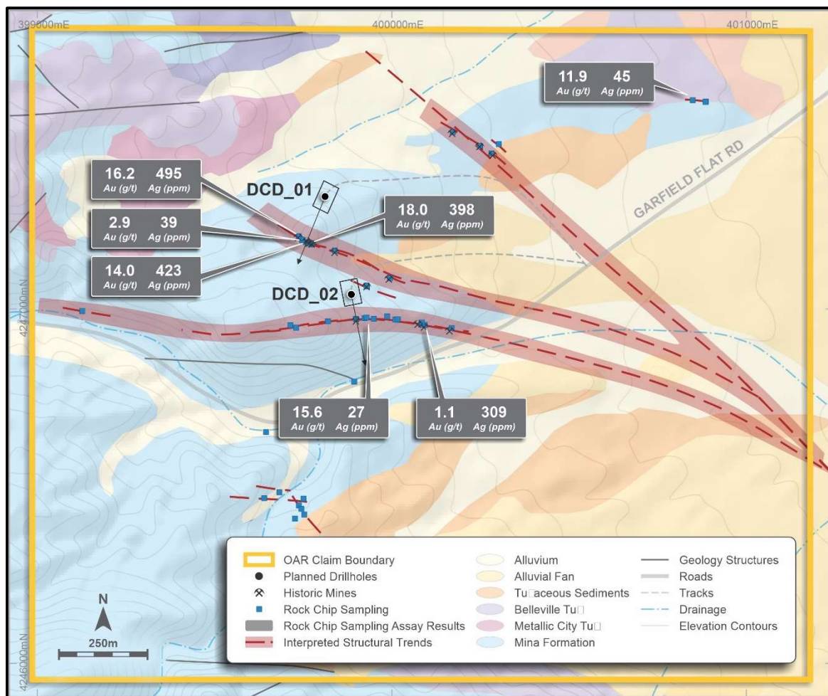
Figure 2: Douglas Canyon Project showing Gold and Silver Sampling Results iii (g/t Au, ppm Ag) and Location of Proposed Stage One Diamond Core Holes
