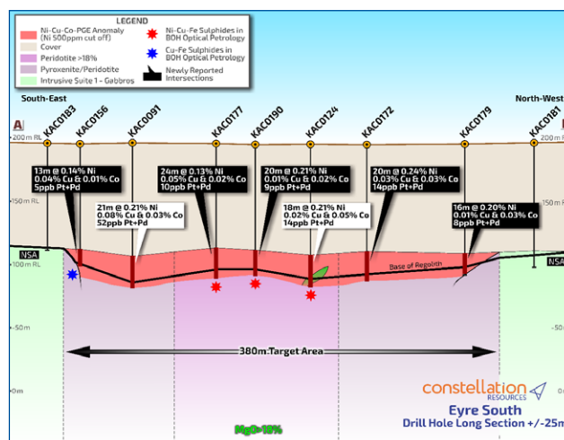
Figure 4. Eyre South Drill Hole Long Section
