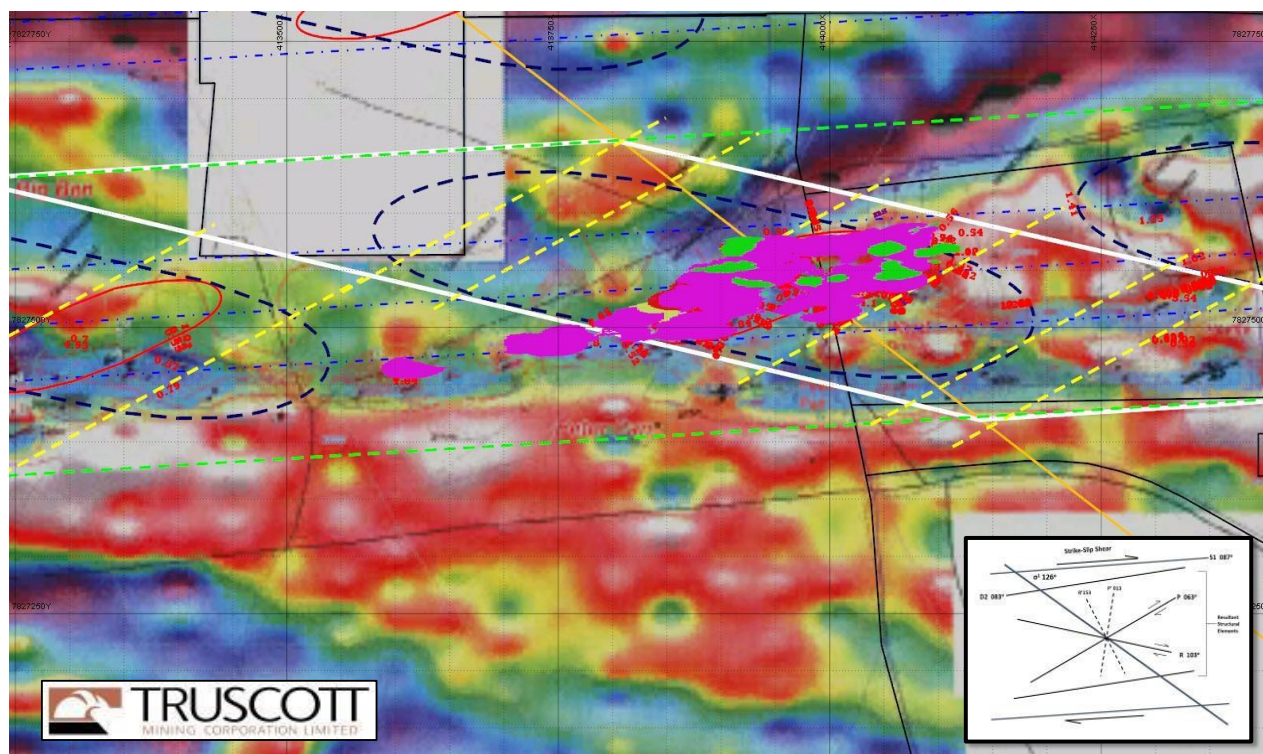
Figure Nine: Ore Body Level (Fractal Four) Westminster – Gold Block Model & Gravity Image
