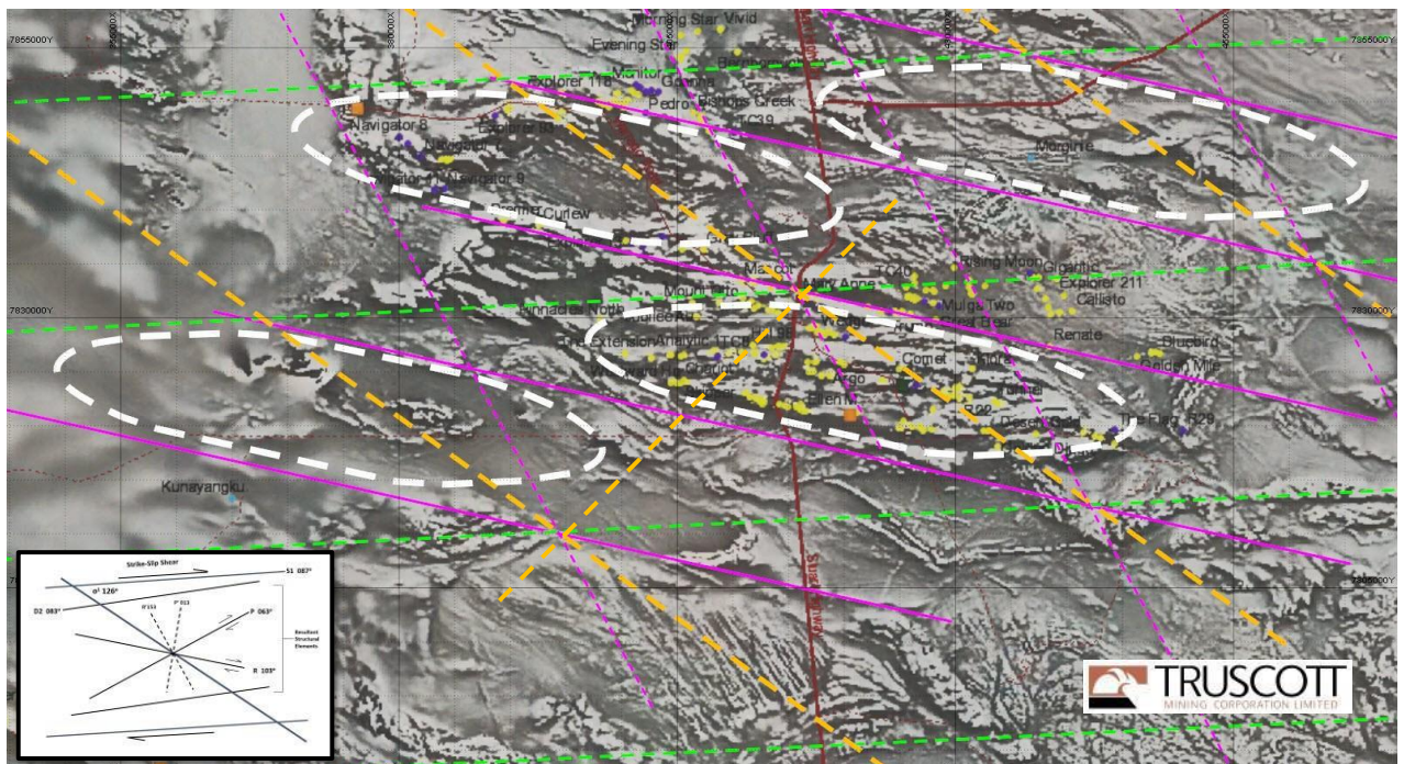
Figure Four: Structural Domains within the Strike-Slip Corridor
