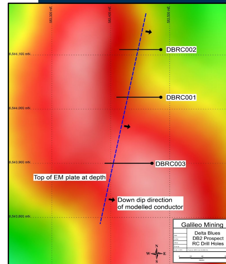
RC Drill Hole Plan Location at Delta Blues DB2 with EM Target over TMI Magnetic Image
