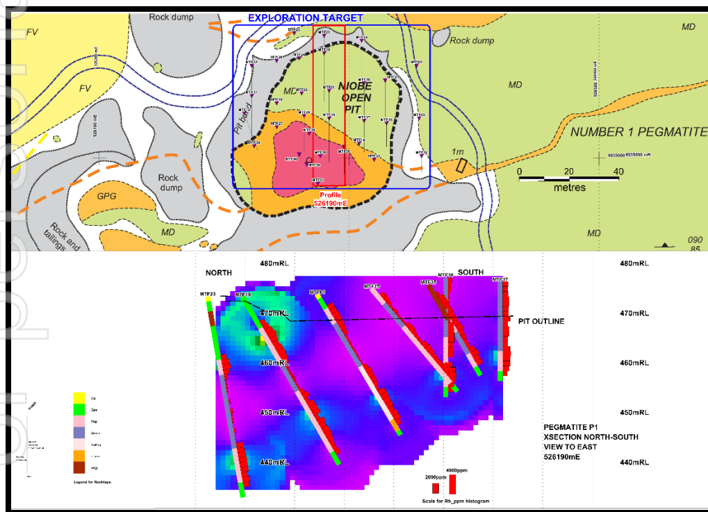
Figure 5: Section 526190mE across the Exploration Target showing the down hole Rubidium assays in both histogram and thematic image as modelled for the Exploration Target
