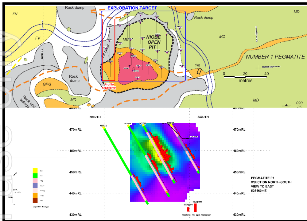
Figure 2: Westerly section (526160mE) across the Exploration Target showing the down hole Rubidium assays in both histogram and thematic image as modelled for the Exploration Target. Key Col- Colluvium, Gab - Gabbro, Peg - Pegmatite, Qcore – quartz core, NaPeg – Sodium Pegmatite, Trans – Transitional lithology, VQZ – massive vein quartz
