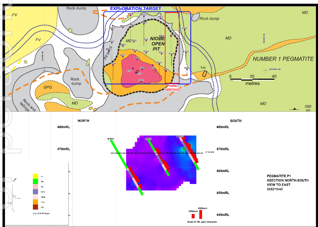
Figure 7: Section 526215mE across the Exploration Target showing the down hole Rubidium assays in both histogram and thematic image as modelled for the Exploration Target
