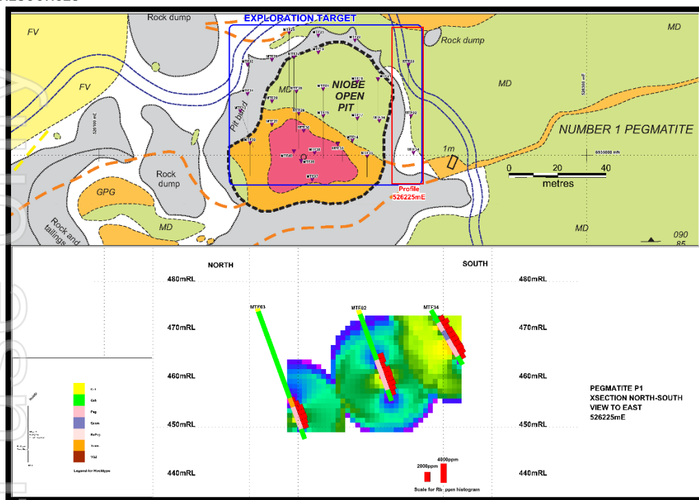
Figure 8: Section 526225mE across the Exploration Target showing the down hole Rubidium assays in both histogram and thematic image as modelled for the Exploration Target.
