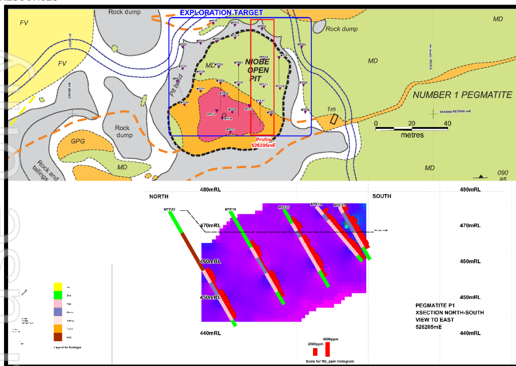
Figure 6: Section 526205mE across the Exploration Target showing the down hole Rubidium assays in both histogram and thematic image as modelled for the Exploration Target
