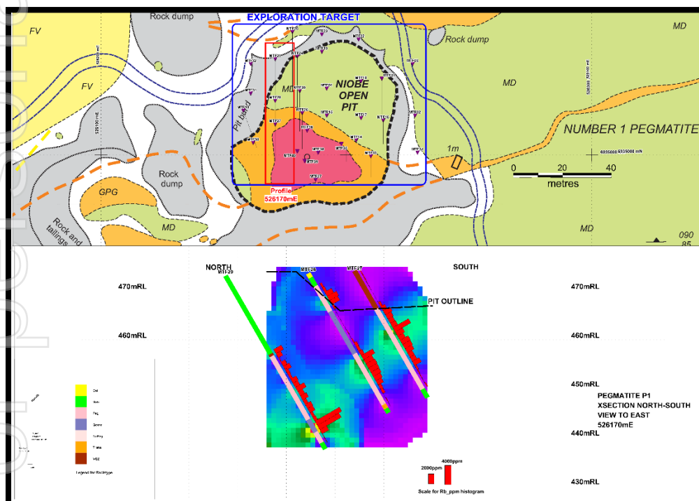
Figure 3: Section 526170mE across the Exploration Target showing the down hole Rubidium assays in both histogram and thematic image as modelled for the Exploration Target
