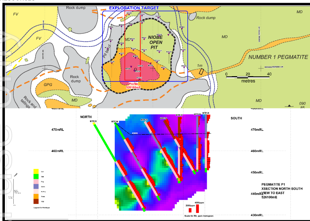
Figure 4: Section 526180mE across the Exploration Target showing the down hole Rubidium assays in both histogram and thematic image as modelled for the Exploration Target
