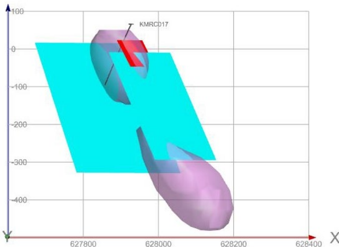
Figure 1: Preliminary modelling of the DHEM (red) and FLEM (2 x blue) plates over the 3D inversion of magnetics at Orion, highlighting that KMRC017 intersected the upper southern corner of the coincident magnetic and EM anomaly.
