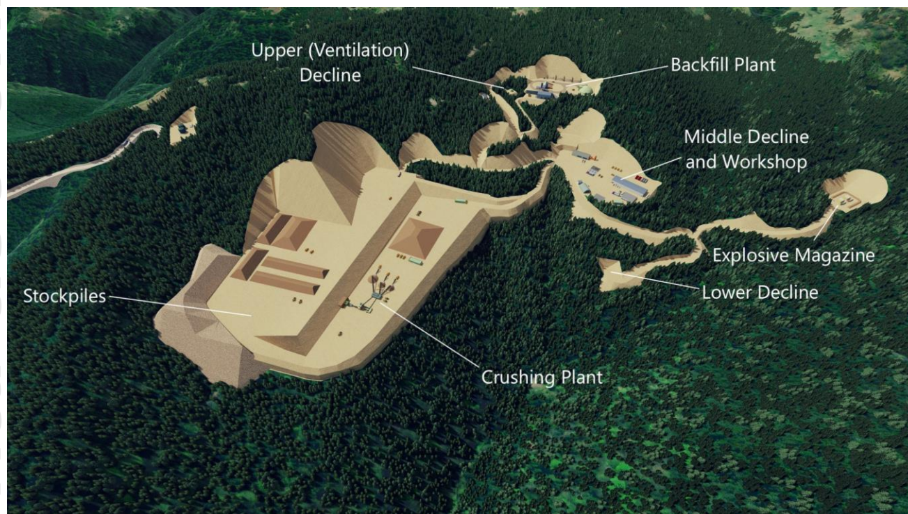
Figure 6: Isometric view of the Rupice Surface Infrastructure showing underground mine plan in red
