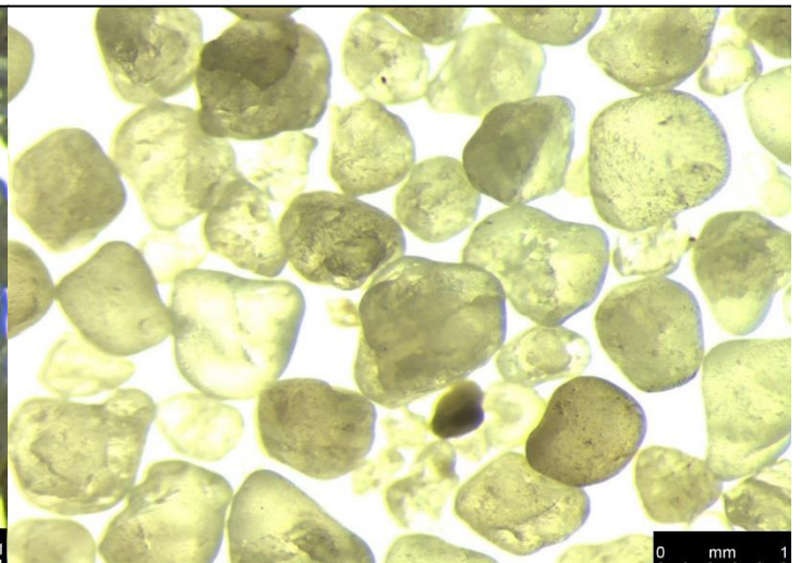
Figure 11: 60 Minute Attrition Product
