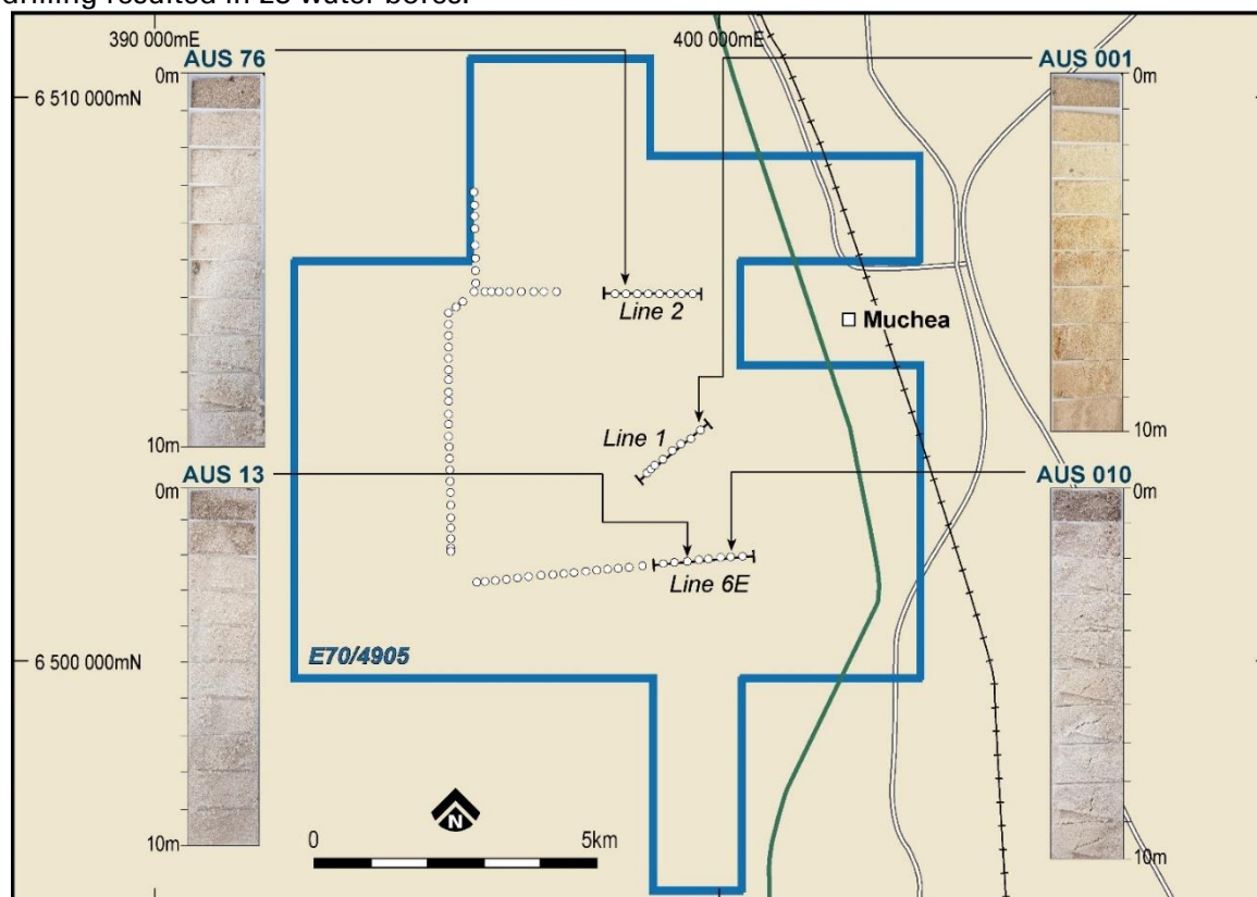
Figure 2: Drill Collar Plan
