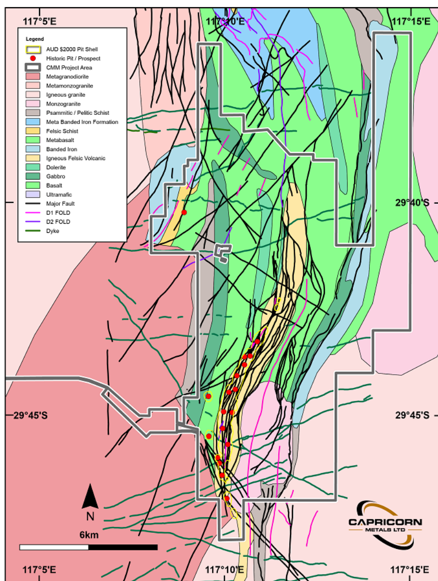
Mt Gibson Gold Project regional geology
