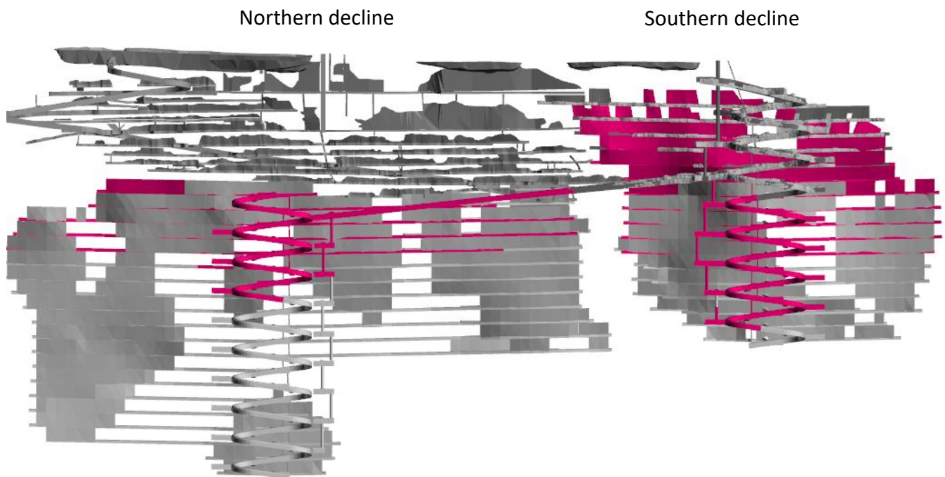
Figure 4: Rothsay long section showing FY22 mine schedule (magenta) v LOM design (looking east)
