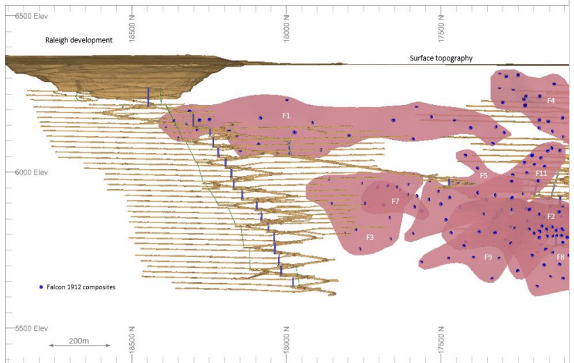
Long section view looking east of the Falcon deposit and data used for estimation
