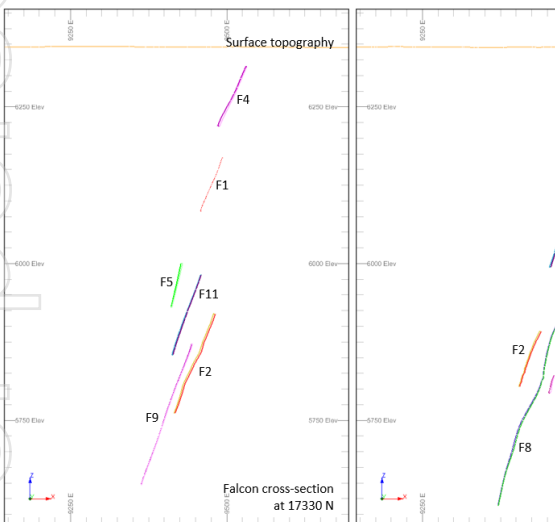
Cross section views of Falcon ore lodes
