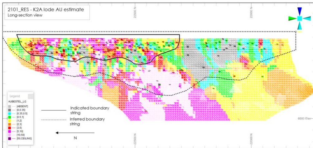
Long section view of the Arctic K2A deposit and the data used in the resource estimate.
