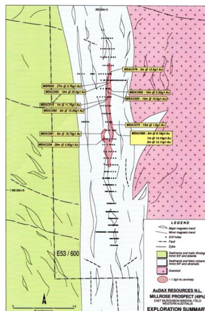
Figure 3: Geological Plan
