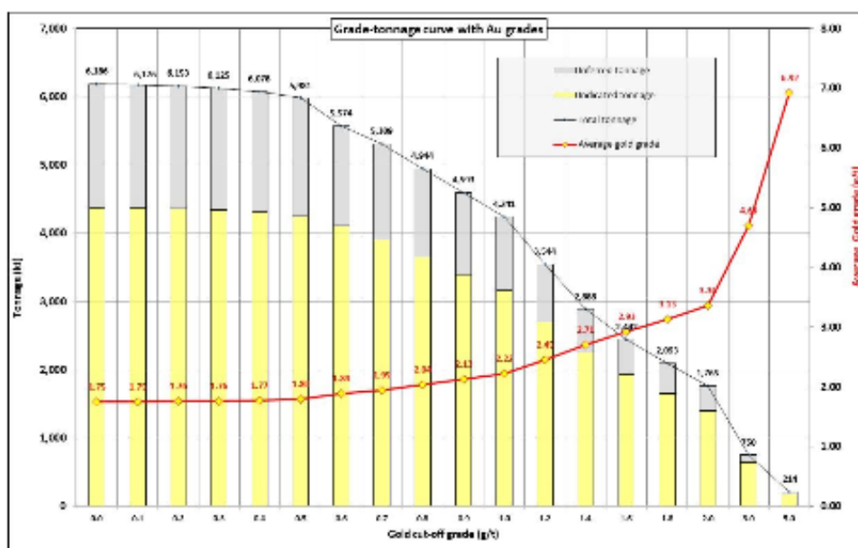
Figure 4: Grade Tonnage curve
