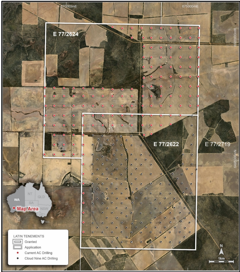
Figure 1: Current drilling program at the Noombenberry Kaolin-Halloysite Project, directly north of the initial Aircore drilling covering the Cloud Nine Deposit.
