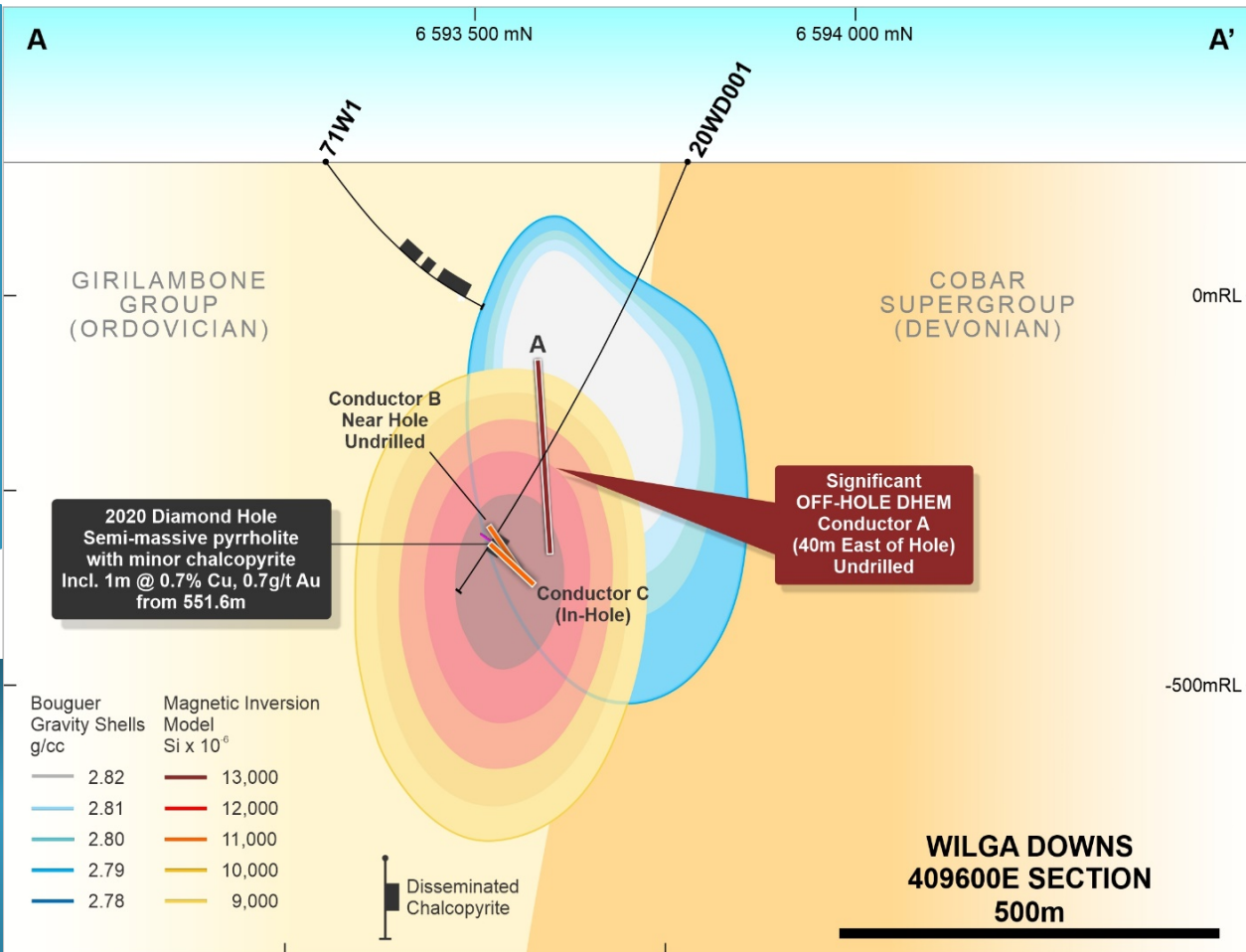
Semi massive pyrrhotite with chalcopyrite from 551.6m (Hole 20WD001). Gold mineralization is also associated with the copper.
