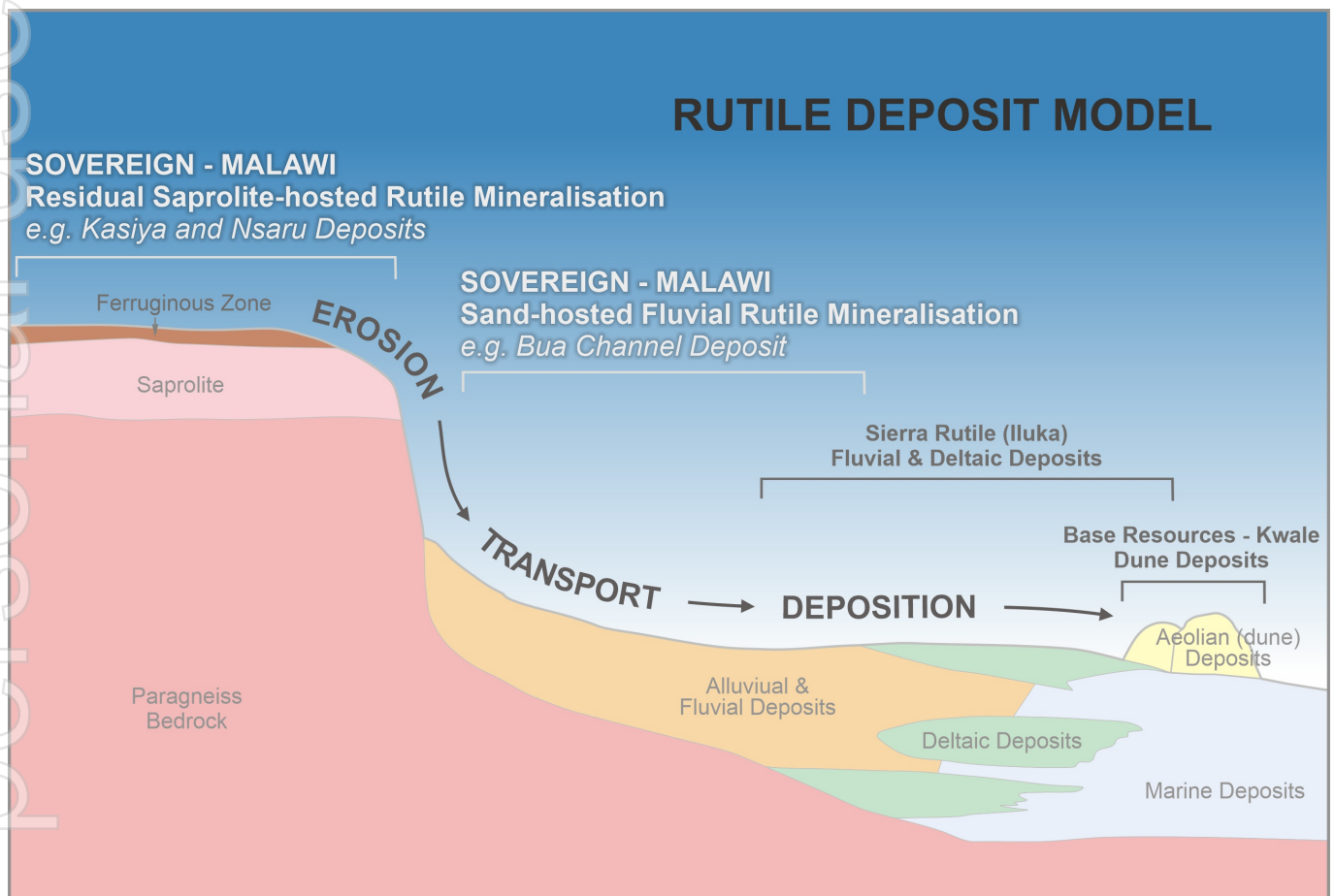
Figure 12: Rutile deposit model showing residual sapolite hosted mineralisation and the various traditional sand hosted deposit types.
