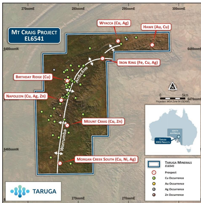
Figure 9: MCCC Project Outline showing Priority Exploration Targets, Historical Copper and Gold Mineral Occurrences & Mines, and the Main Structural Feature being the Worrumba Anticline.
