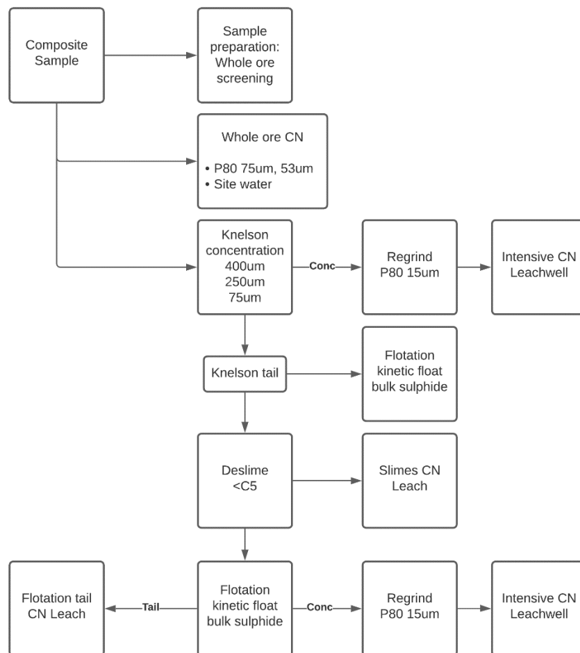
Figure 2: BT1A composite silver recovery test work program flow sheet undertaken by ALS, Burnie.
