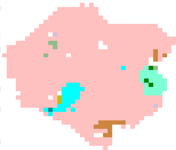
Figure 3: Back Scatter Electron micrograph (top) and QEMSCAN false colour particle image (lower) of silver hosted in quartz particle for BT1A flotation tail leach residue from analysis completed by Bureau Veritas Mineralogy, Adelaide.
