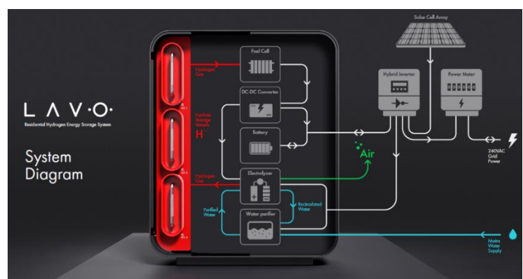
Figures: LAVO 40 kWh Hydrogen Battery and System Diagram, planned for installation at Ularring
