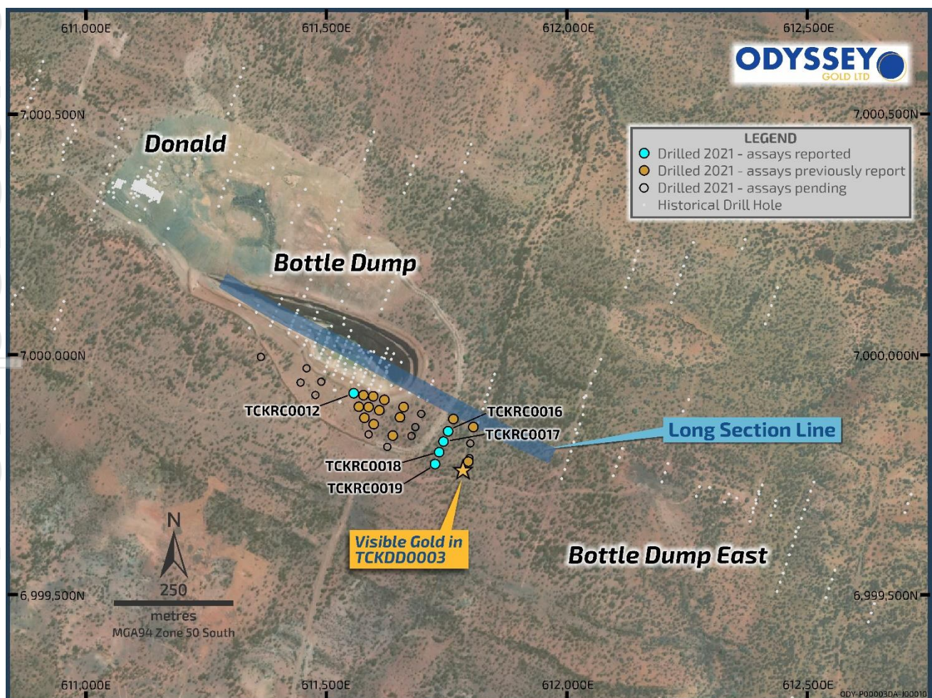
Figure 4. Planned and previous drill holes across the Bottle Dump area.
