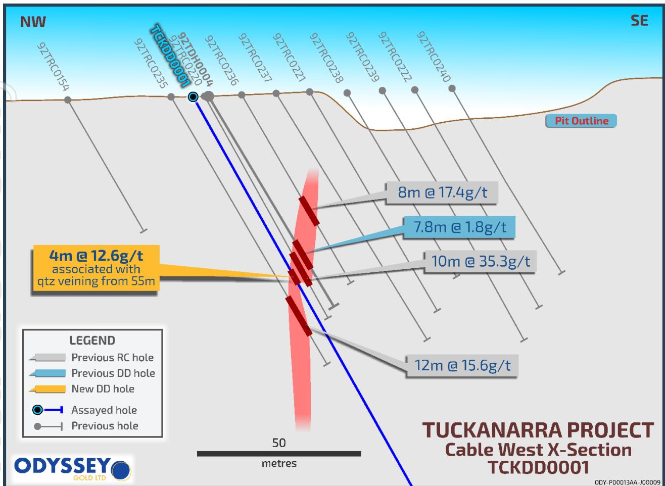
Figure 7. Cross-section of first diamond hole at Cable West with historical results.
