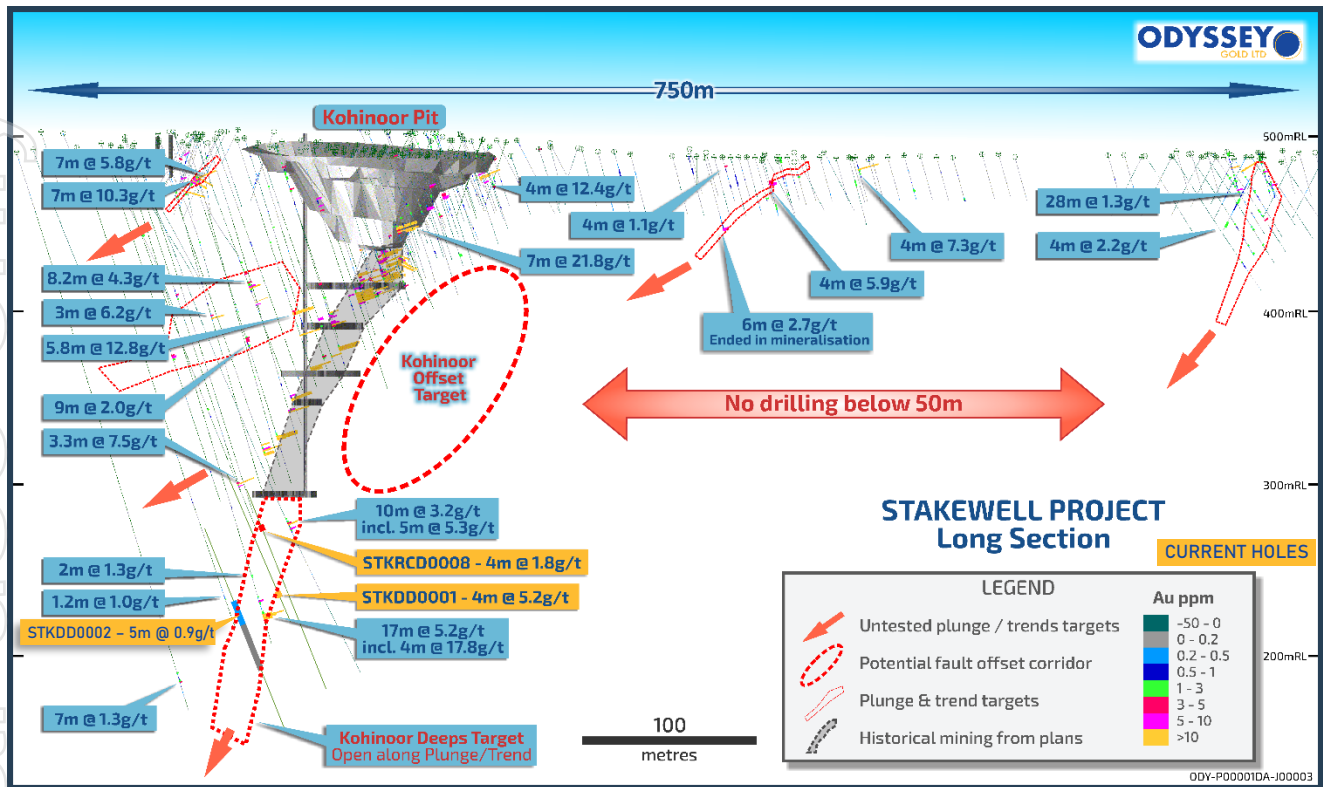
Figure 9. Stakewell targets showing recent diamond drilling.
