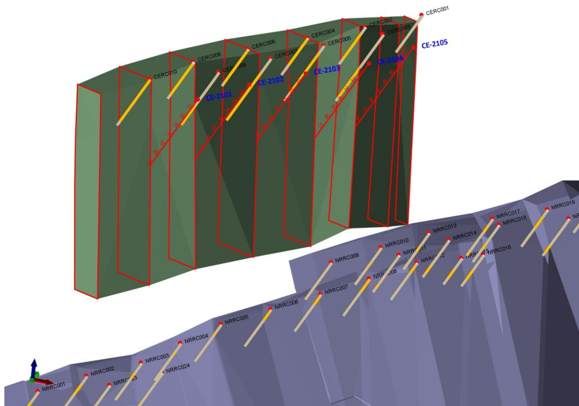
Figure 2. Centurion (background) and Northern Reward (Foreground) Exploration Target wireframes defined on historic drillholes (beige) and planned resource drillholes (red).
