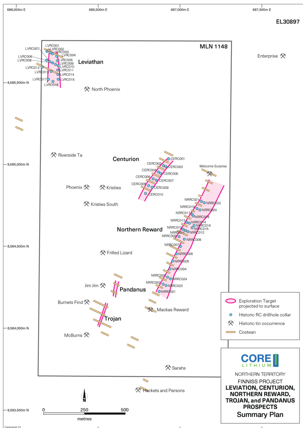
Figure 3. Leviathan Group of Lithium Exploration Target and Historic Drilling, ML 1148
