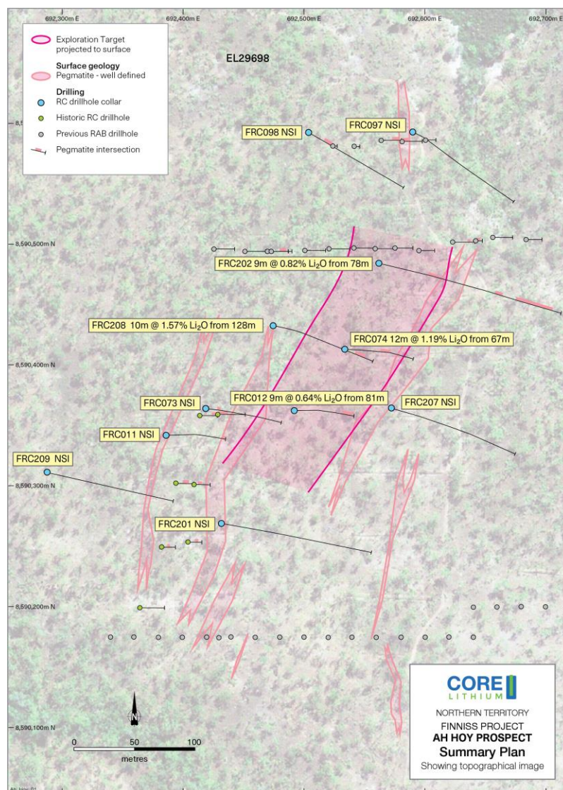
Figure 6. Ah Hoys Lithium Exploration Target and previous Core drilling.
