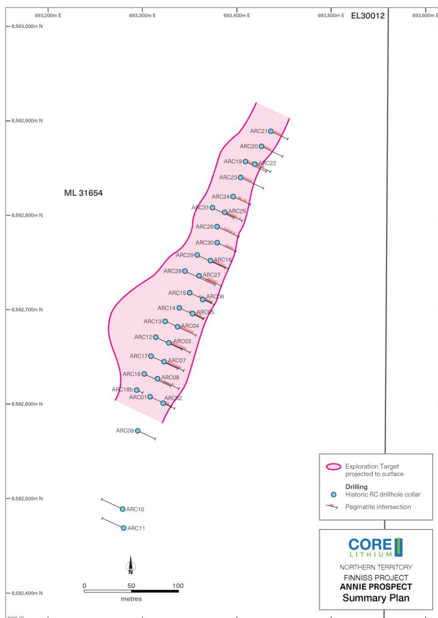
Figure 4. Annie Lithium Exploration Target and Historic Drilling
