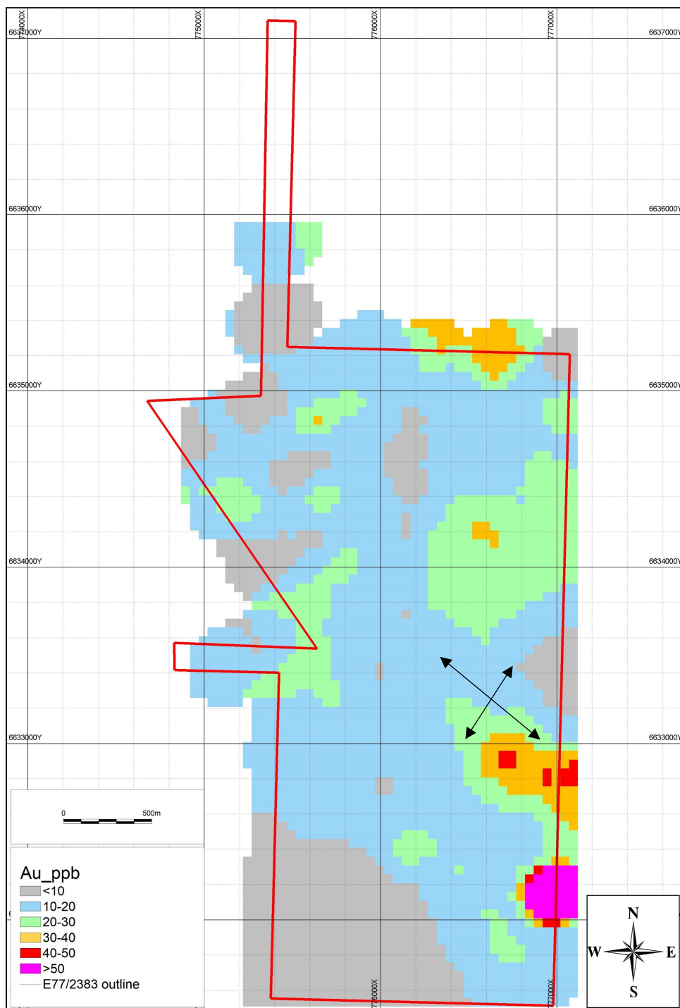
Figure 3: Soil geochemical map colored by Au ppb showing anomalous which is approximately 800x500m
