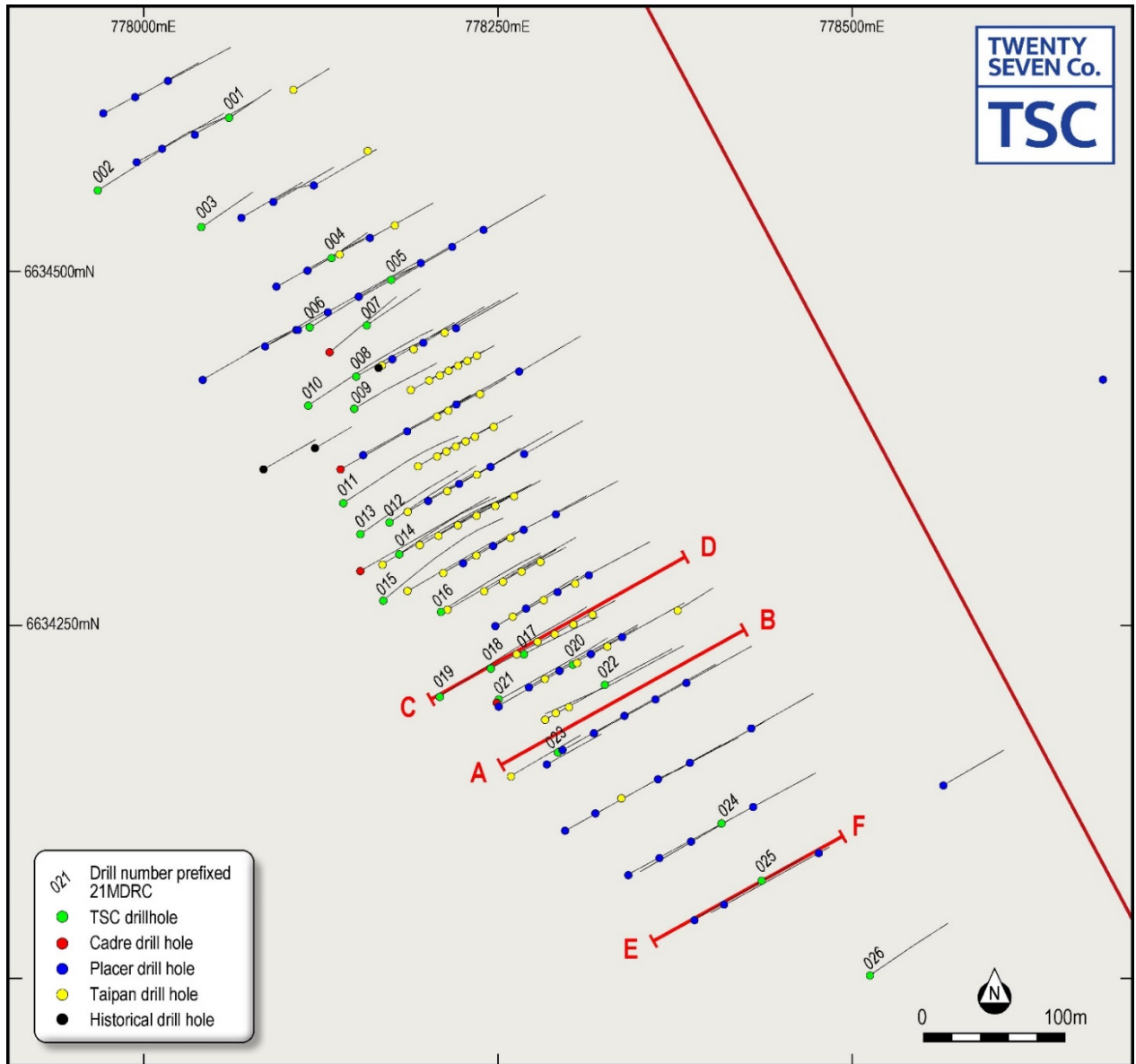
Figure 4: Map showing the Locations of TSC drill holes and the cross section location
