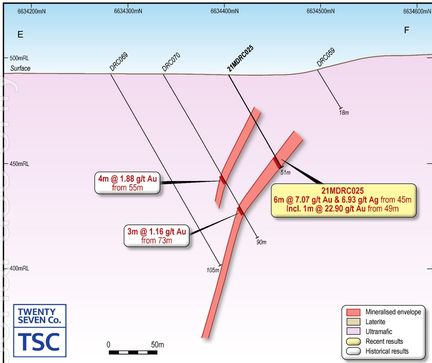
Figure 2: Cross Section showing historical results in white and recent results in yellow
