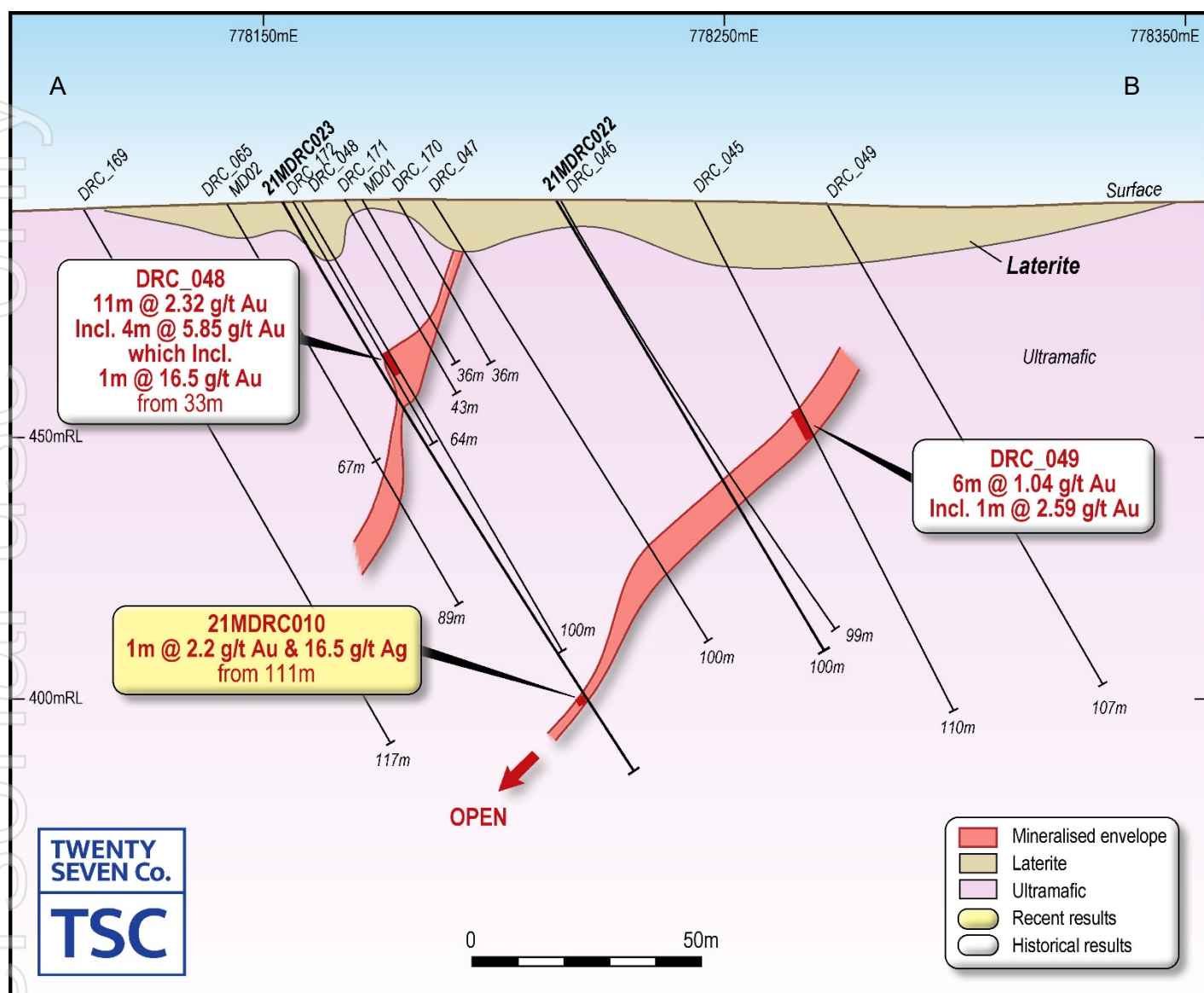
Figure 1: Cross Section showing historical results in white and recent results in yellow
