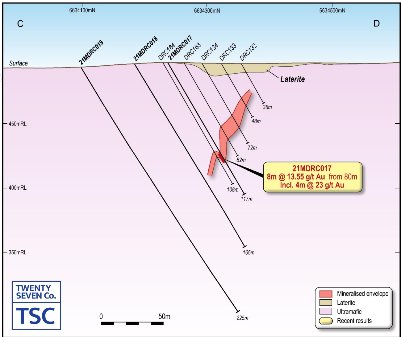
Figure 3: Cross Section showing historical results in white and recent results in yellow
