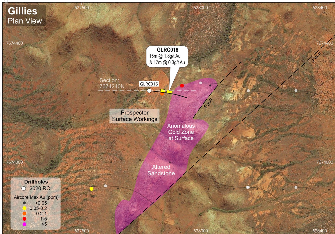
Figure 2: Plan of Gillies showing anomalous gold in drilling
