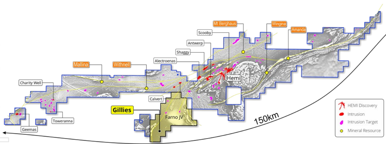
Figure 1: Location diagram of Gillies, within De Grey's tenement holdings, Pilbara WA
