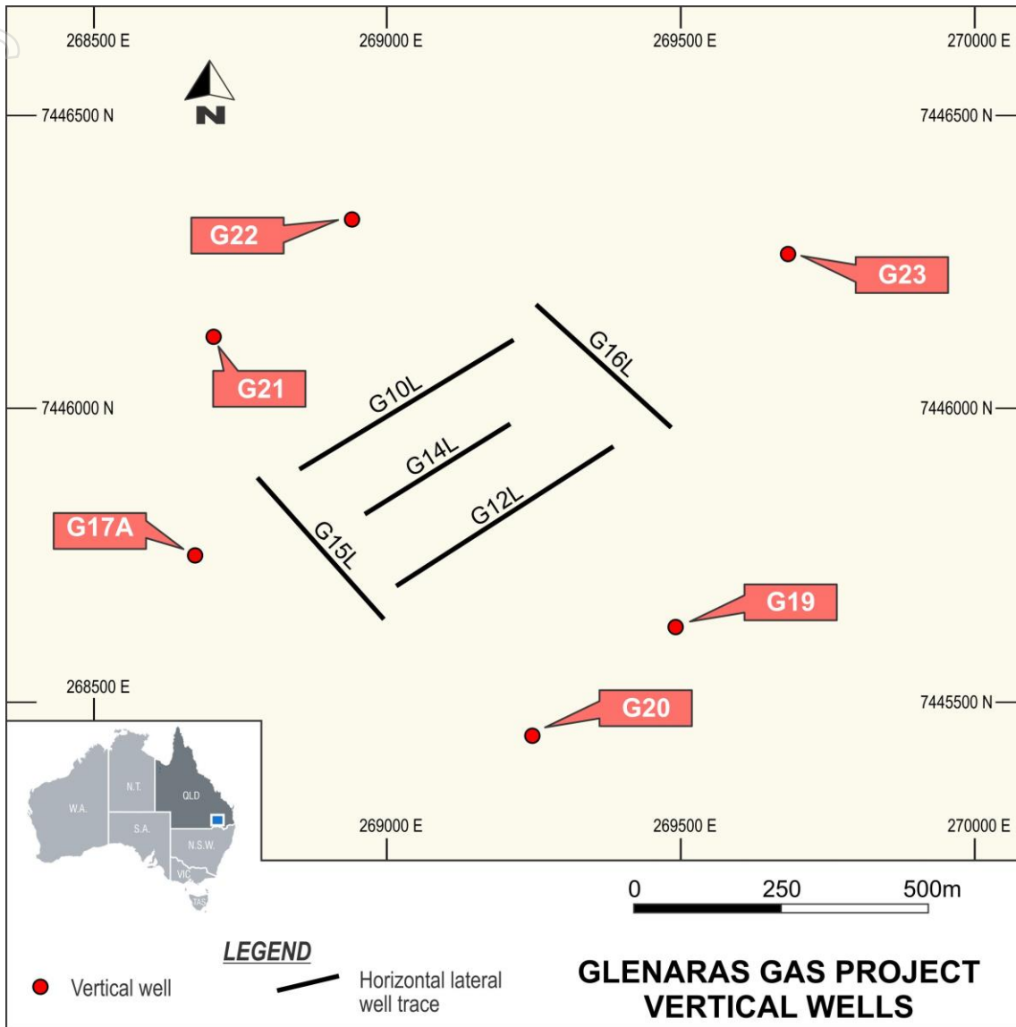
Figure 1 – New vertical well locations.
