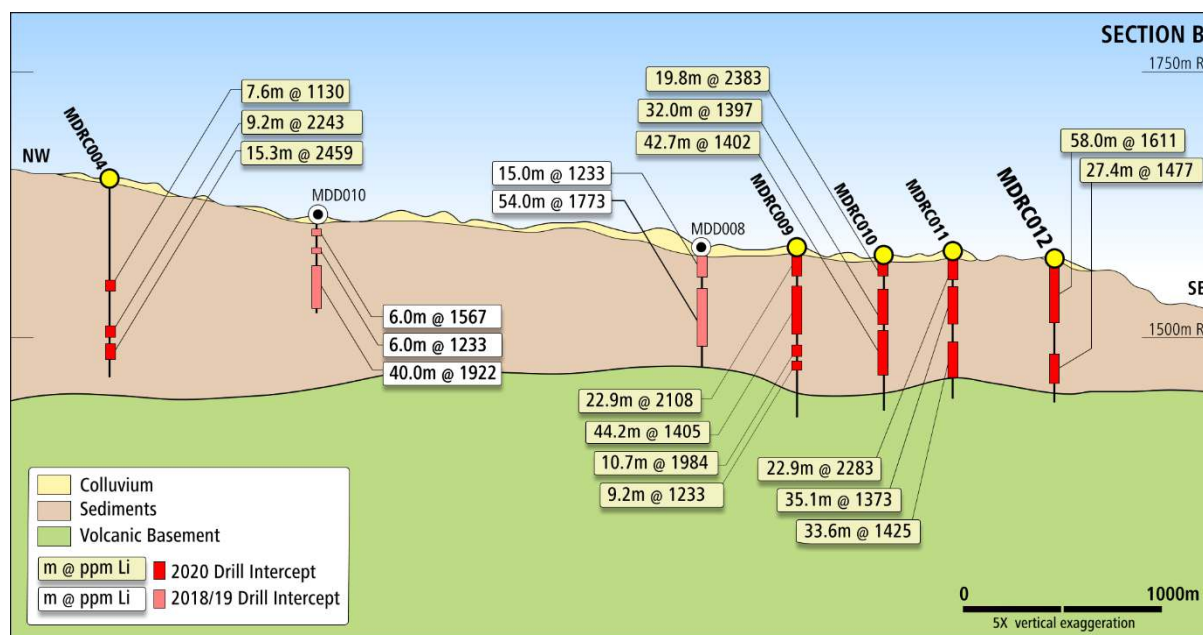
Figure 1 – Schematic section showing significant intercepts through the McDermitt Project.
