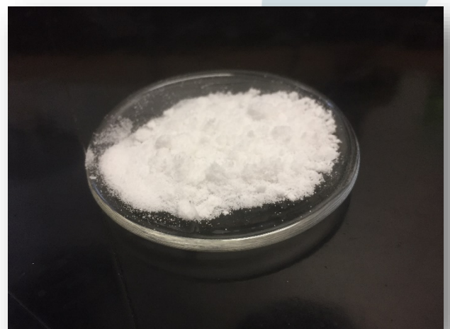
Image 1: Lithium Carbonate
