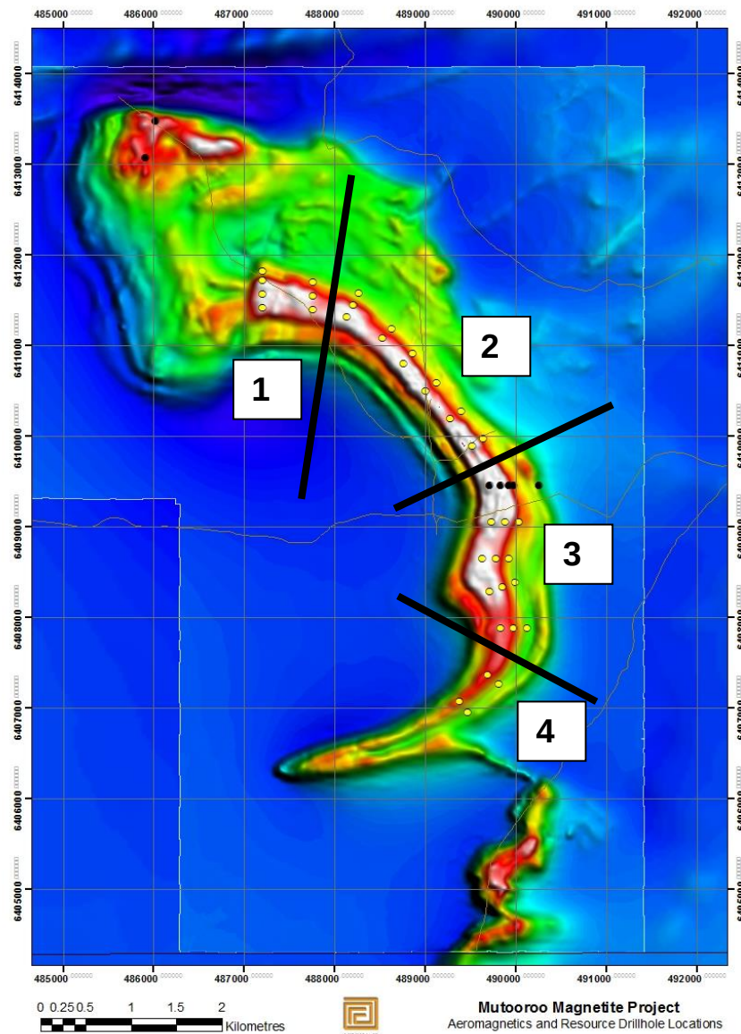
Figure 6 Muster Dam Prospect Modelling Sub-divisions
