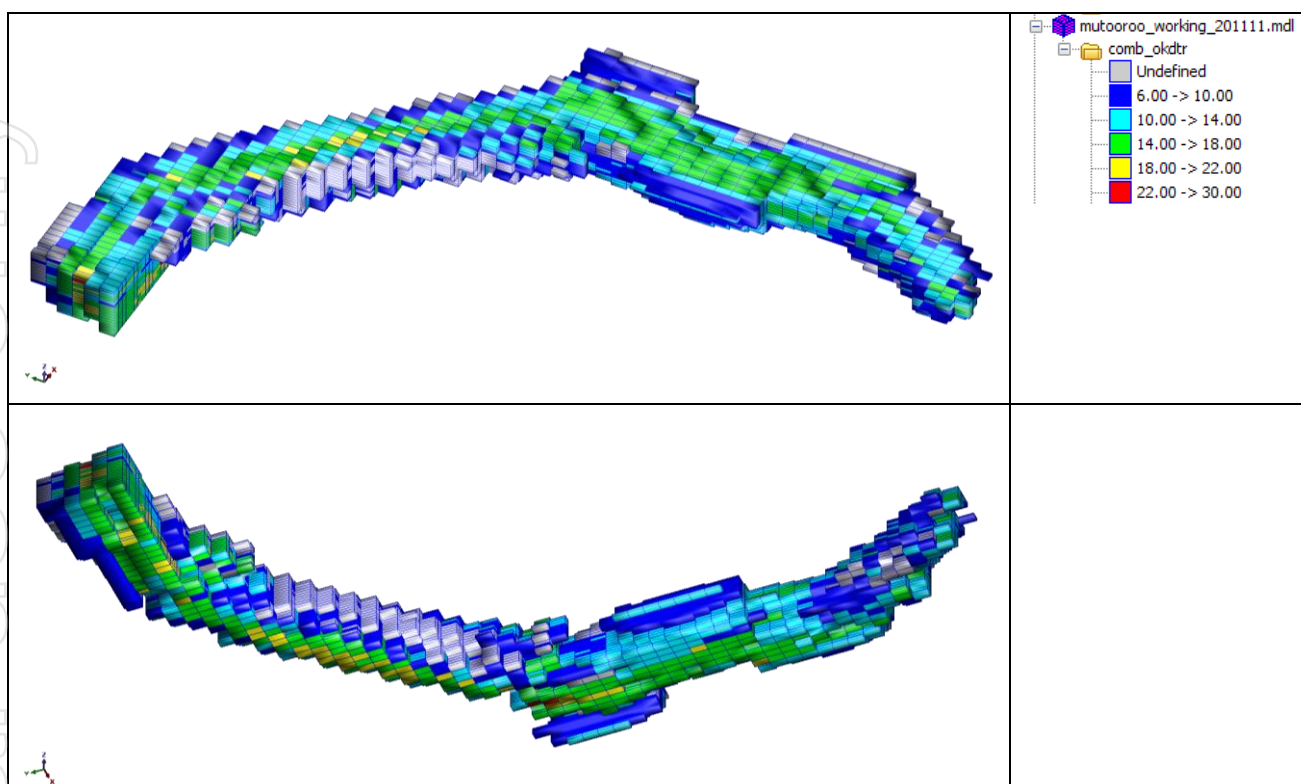
Figure 9 Muster Dam Prospect DTR Magnetite Grade Distribution
