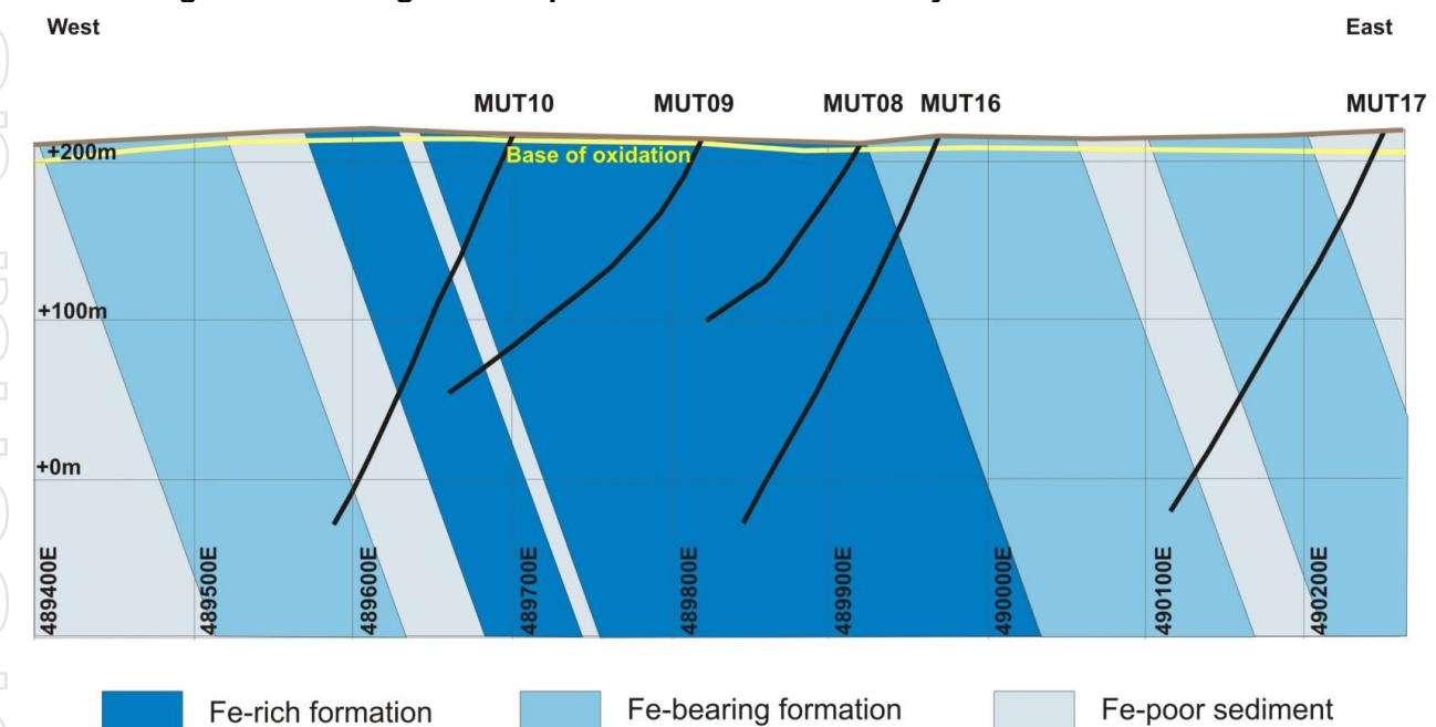
Figure 3 Geological Interpretation of the Discovery Section at Muster Dam
