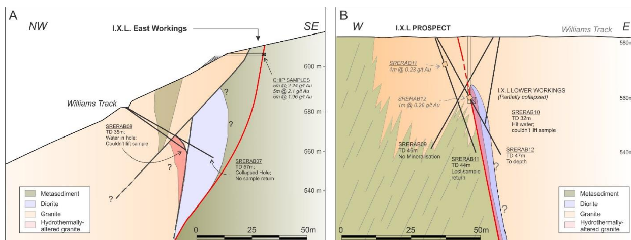
Figure 5: A) Cross-section showing drill holes SRERAB07 and SRERAB08 across the IXL East prospect with preliminary geological interpretation. Chip samples noted are reported in Dart ASX July 2020 . B) Cross-section drill holes SRERAB09-SRERAB12 across the IXL Prospect. No mineralised intercepts were recovered from either the IXL or IXL East prospect.
