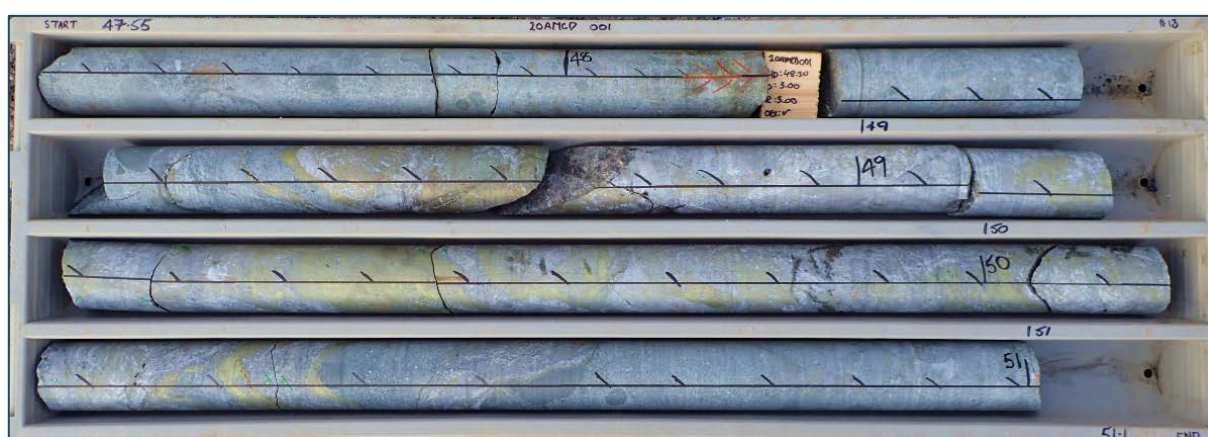
Figure 1: Semi-massive to stringer chalcopryrite mineralisation within chlorite altered fragmental rhyolite in 20AMCD001.
