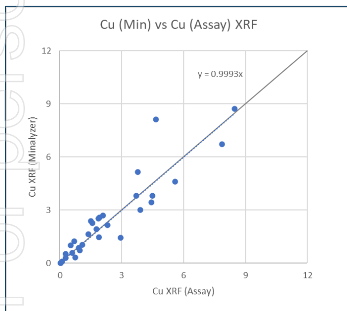
Figure 6: Cu-grades of selected calibration samples.
