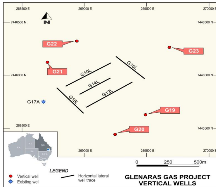
Figure 1 – New vertical well locations
