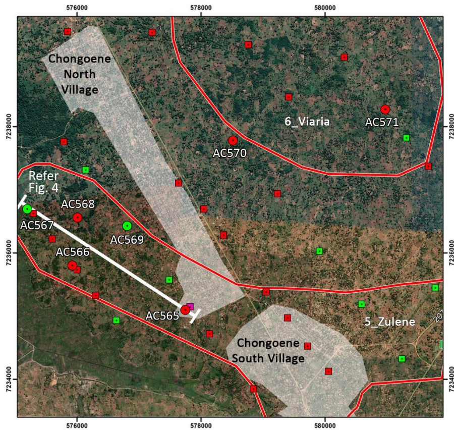
Corridor South Project, Zulene and Viaria Lab results of aircore, December 2020
