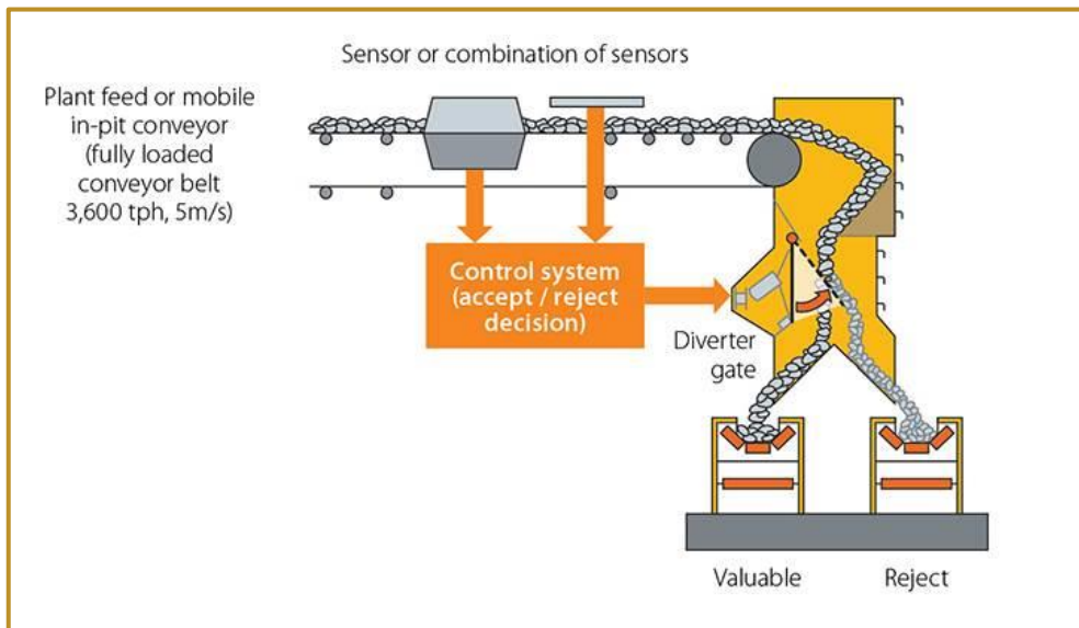
Figure 1: Schematic of bulk ore sorting
