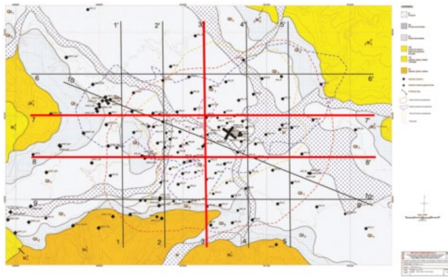
Figure 3. Deposit geological map and cross sections 3, 7 and 8
