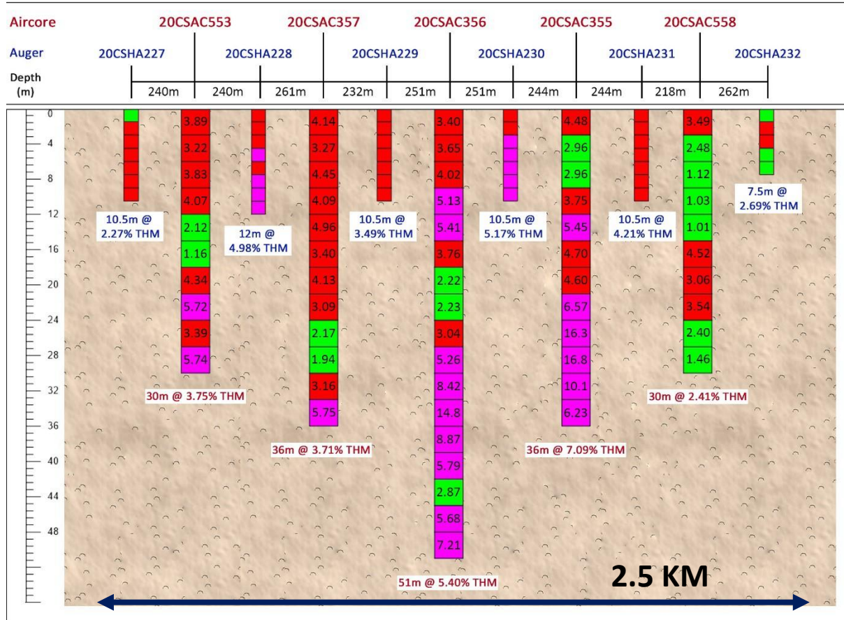
Figure 4. Cross section showing aircore and hand auger holes drilled in the infill auger program (20CSHA227, '228, '229, '230, '231 and '232; refer ASX Announcement 11 June 2020); Poiombo Phase 1 (20CSAC357, '356 and '355; refer ASX Announcement 18 June and 19 June 2020) and Phase 2 programs, % THM results for each sample intersection and the average of the entire drillhole is shown. Due to vertical exaggeration elevation not presented.
