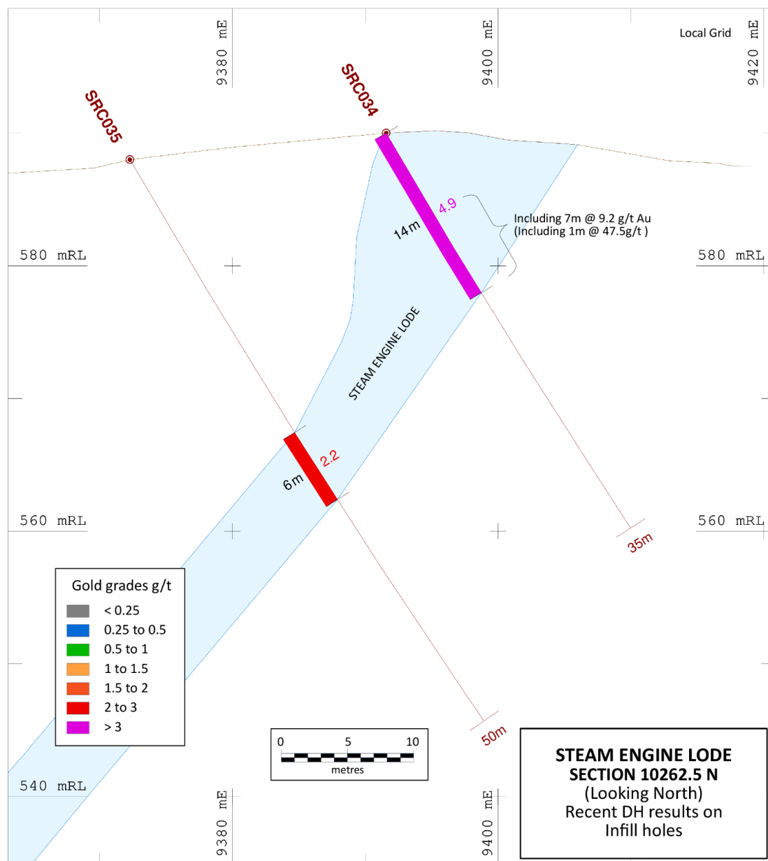
Figure 3. Cross Section 10262.5 N (local grid) on the Steam Engine lode showing the significant intersections. Mineralisation and grade intersections are shown as colour-coded bars.
