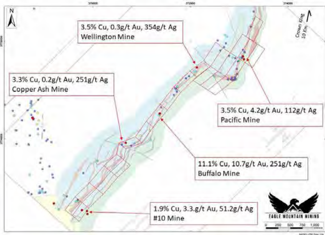
Figure 10 - Results of historical mine dump samples at the Pacific Horizon prospect.
